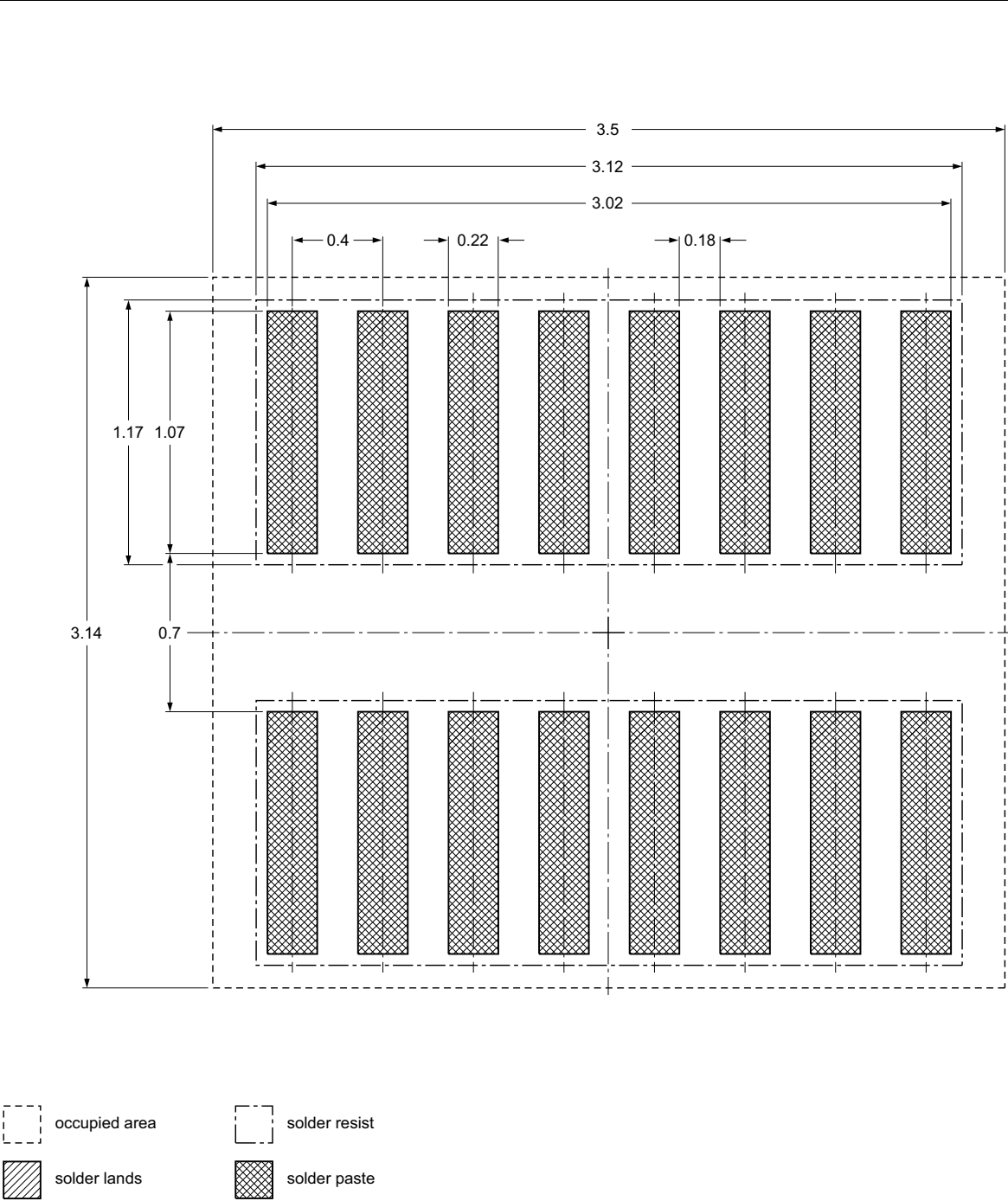
Footprint information for reflow soldering of XSON16 package
