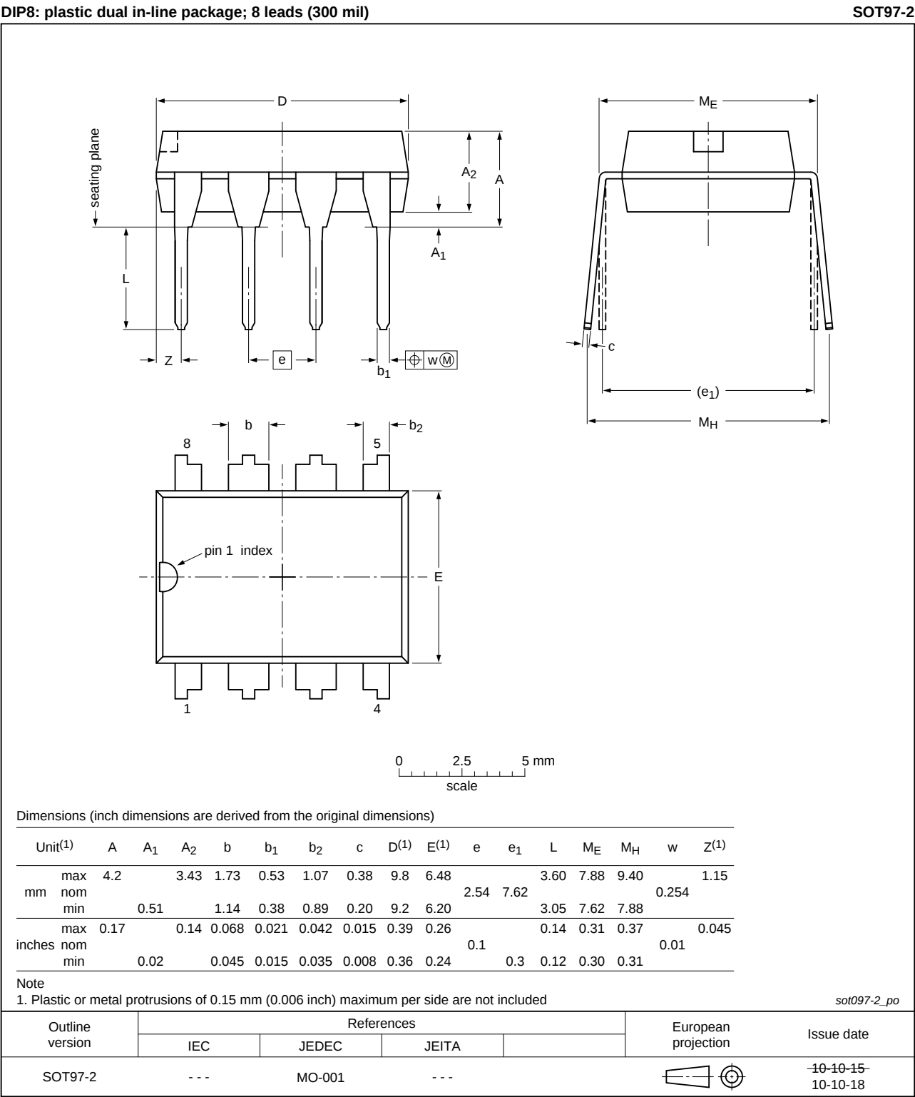
Fig 38. Package outline SOT097-2 (DIP8)
