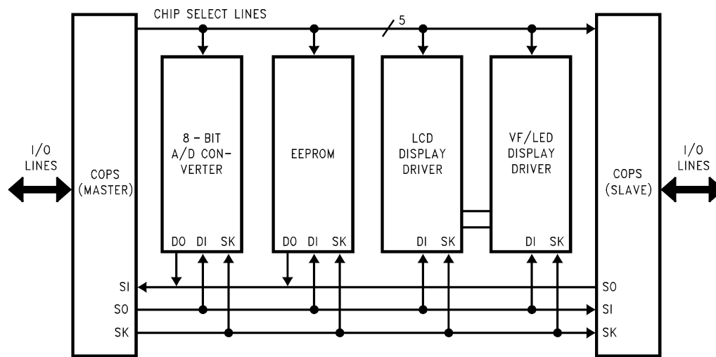
FIGURE 24. MICROWIRE/PLUS Application
