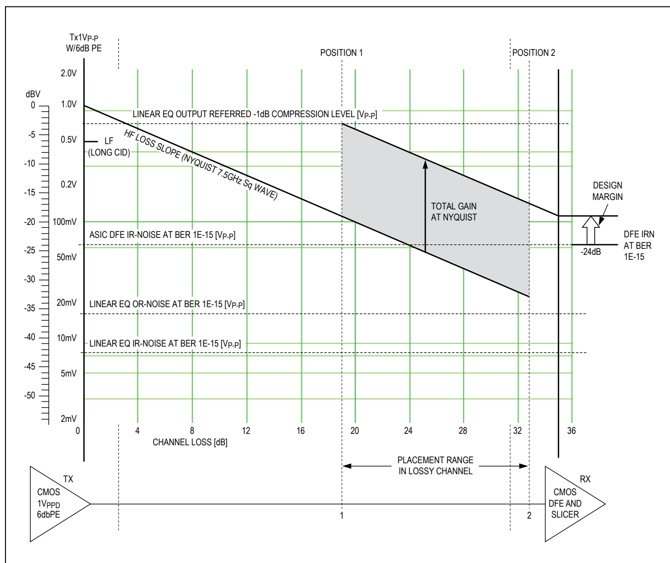
Figure 5. Linear Equalizer Placement
