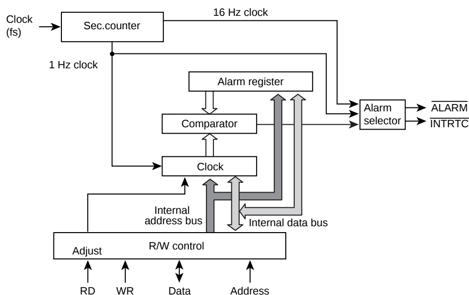
Figure 14-1 Block Diagram
