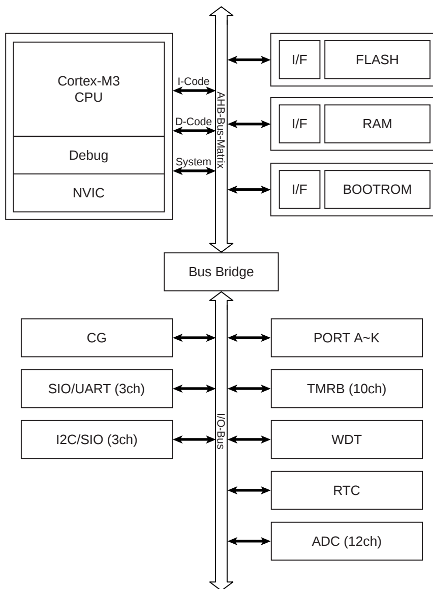
Figure 1-1 TPM333FDFG/FYFG/FWFG Block Diagram
