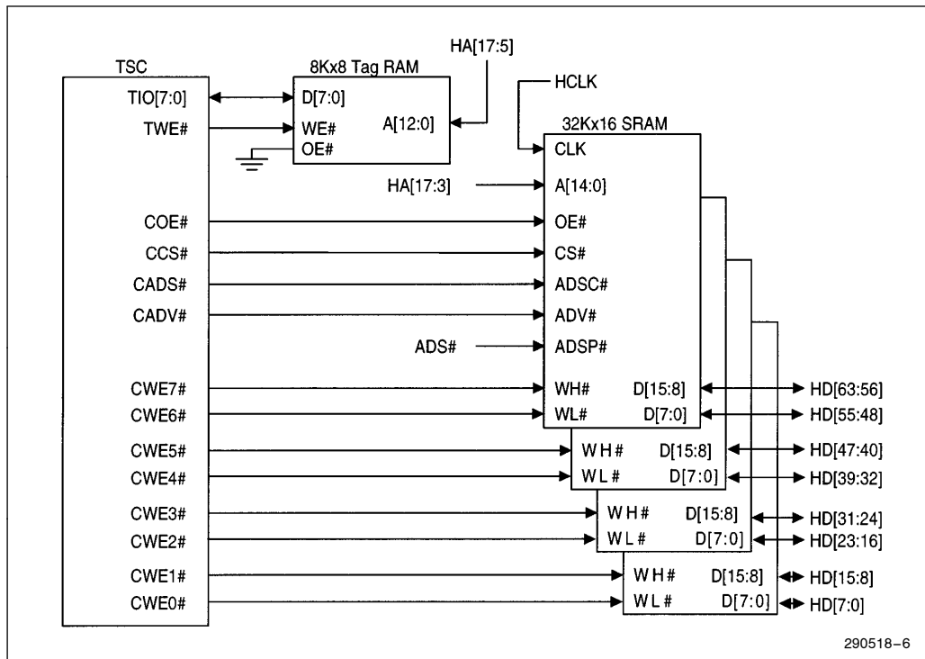
Figure 4. 256-Kbyte Second Level Cache (Burst SRAM)
