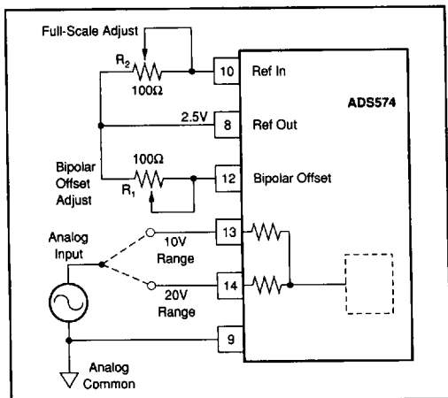
FIGURE 11. Bipolar Configuration.
