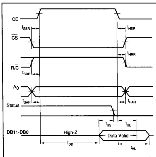
FIGURE 6. Read Cycle Timing.
