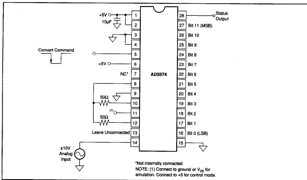
FIGURE 2. Basic ±10V Operation.
