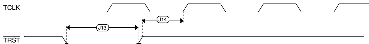
Figure 9. Test Access Port timing
