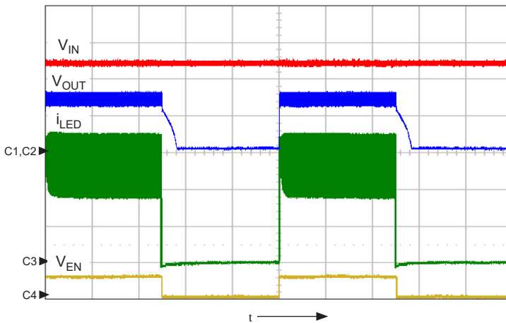
Panel 15A: Operation without using any output capacitor across the LED string
