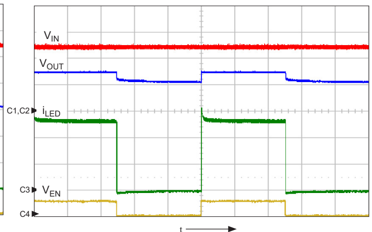
Panel 15B: Operation with a 0.68 \mu\text{F} ceramic capacitor connected across the LED string
