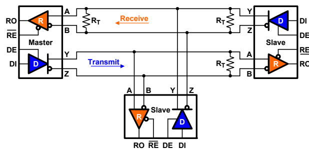
Figure 38. Full-Duplex Bus
