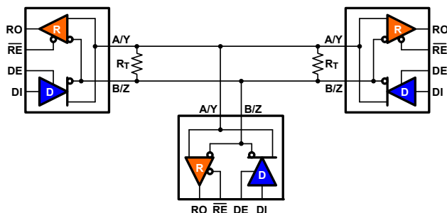
Figure 37. Half-Duplex Bus
