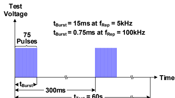
Figure 36. EFT Test Timing
