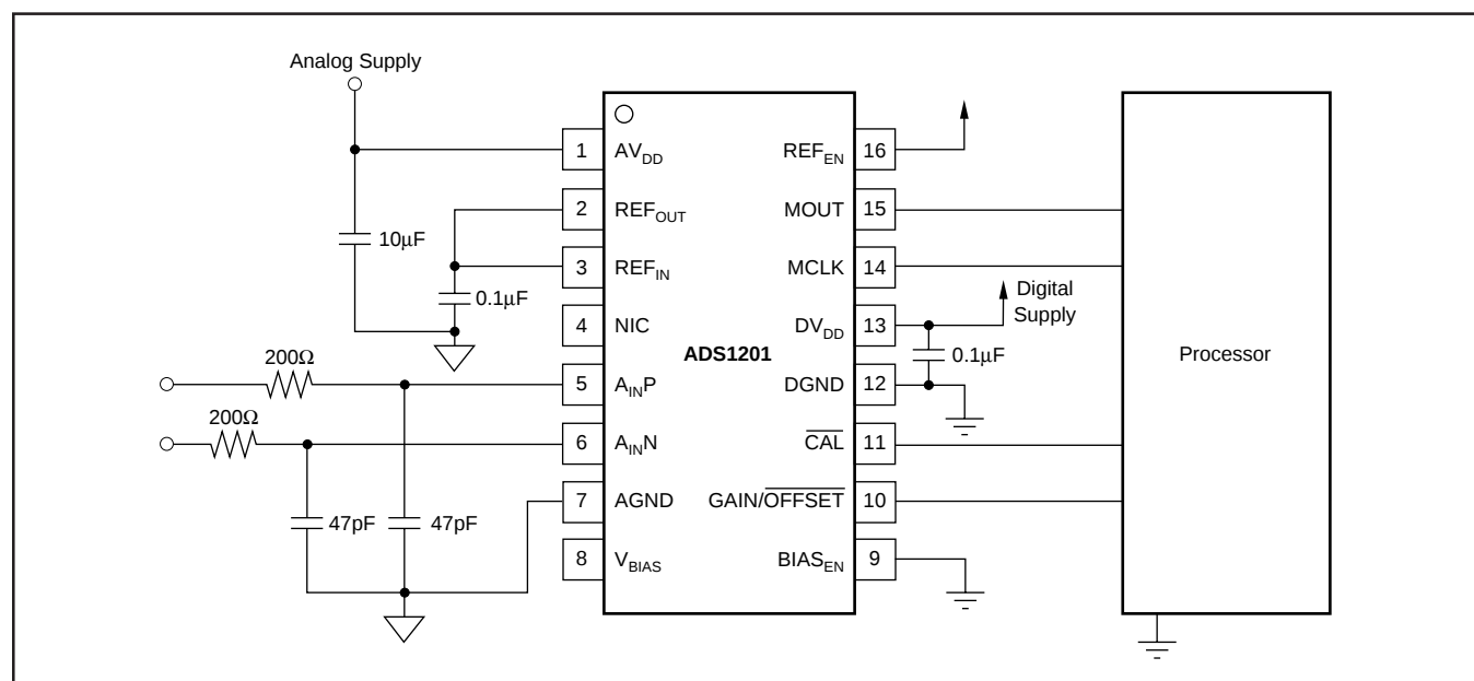
FIGURE 1. Connection Diagram for the ADS1201 Delta-Sigma Modulator Including External Processor.
