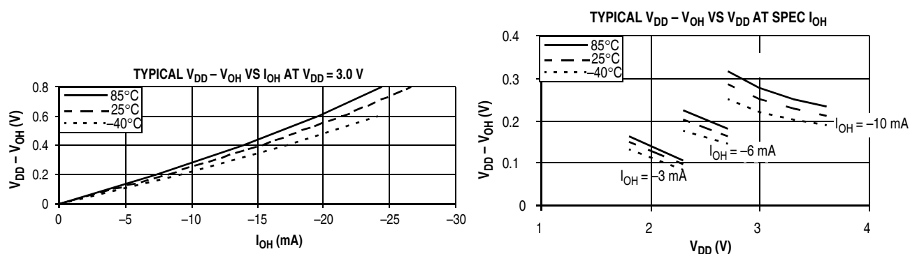
Figure A-5. Typical High-Side (Source) Characteristics — High Drive (PTxDSn = 1)
