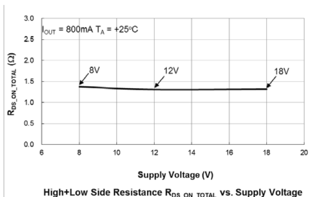
Total H-Bridge Path Resistance – Total R_{DS(ON)} of High-Side and Low-Side Switches
