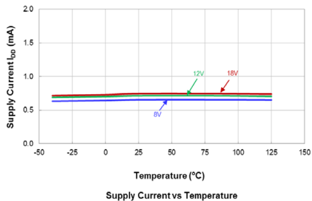
Average Supply Current
