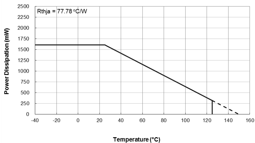
PDIP-8 Thermal Derating Curve
