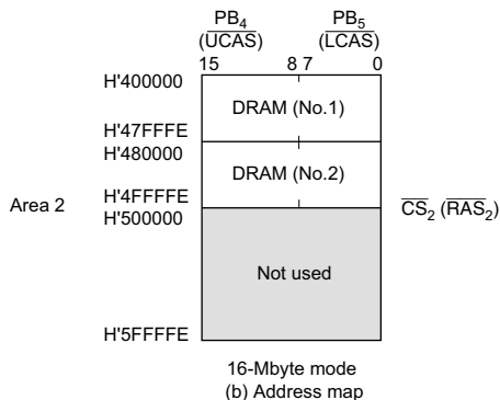
Figure 6.33 Interconnections and Address Map for 2-CAS 4-Mbit DRAMs with \times 16-Bit Organization
