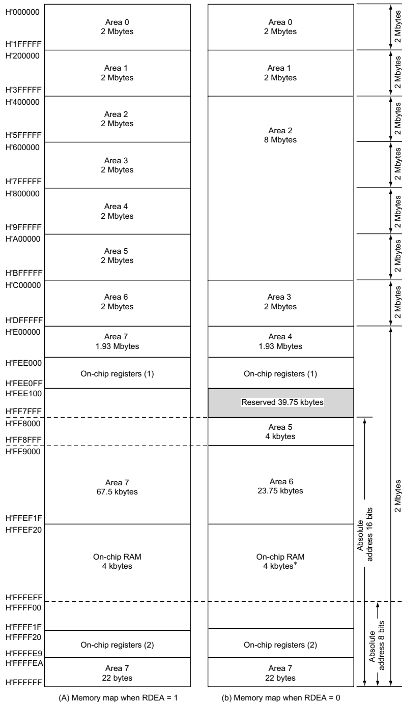
Figure 6.3 Memory Map in 16-Mbyte Mode
