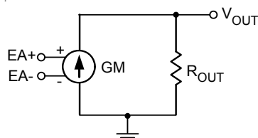
Figure 6. OTA Topology
