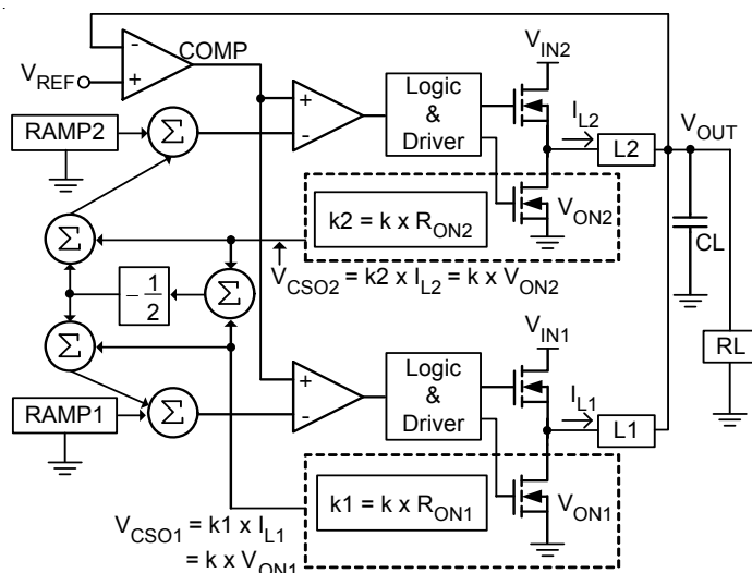
Figure 5. Current Balance
