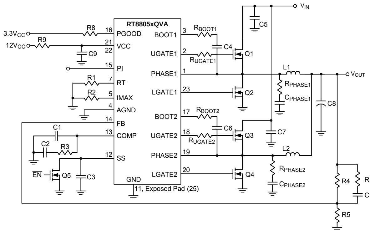
Figure B. Application Circuit for RT8805xQVA (VQFN-24L 4x4)-Standalone Mode (PI Disabled)
