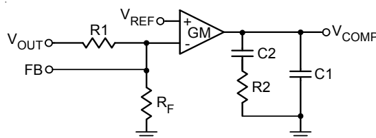
Figure 7. Compensation Loop
