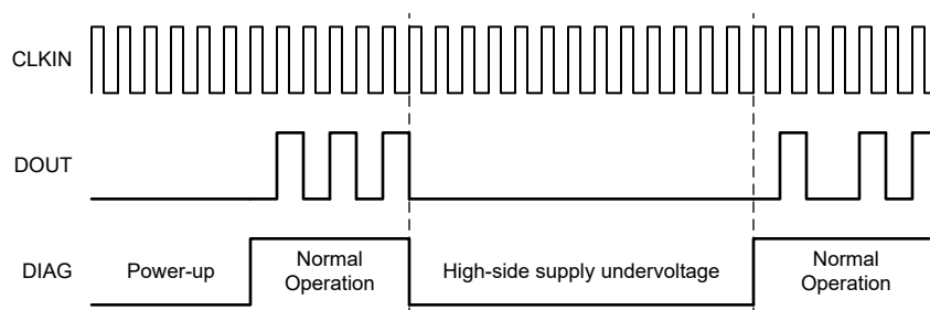
Figure 7-7. DIAG and Output under Different Operating Conditions
