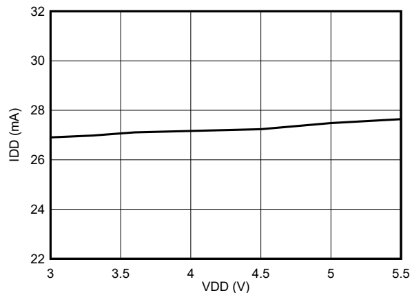
Figure 6-39. Supply Current vs Supply Voltage
