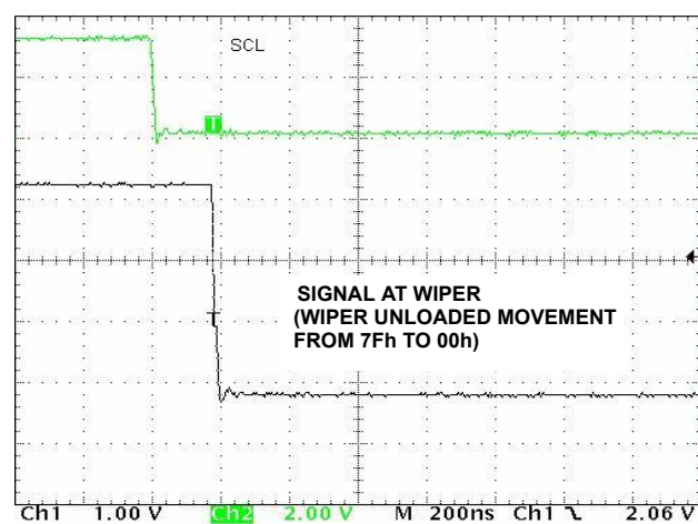
FIGURE 10. LARGE SIGNAL SETTLING TIME
