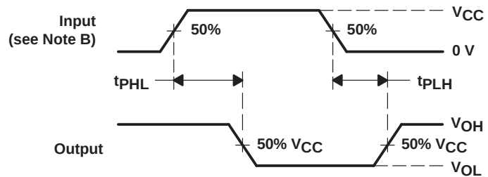
VOLTAGE WAVEFORMS
