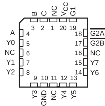
54AC11238 . . . FK PACKAGE (TOP VIEW)
