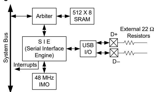
Figure 7-16. USB
