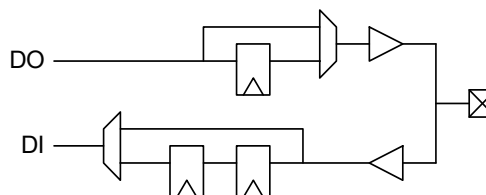
Figure 7-11. I/O Pin Synchronization Routing
