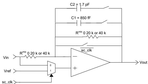
Figure 8-13. Mixer Configuration
