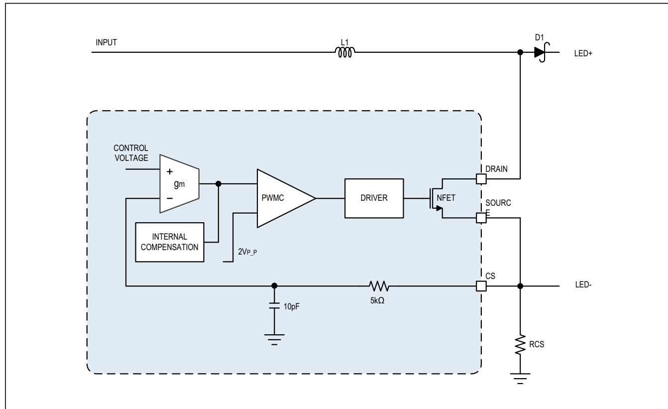
Figure 1. Control Loop
