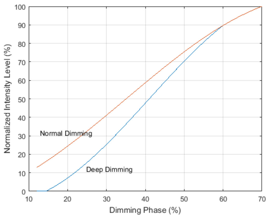
Figure 3. Deep Dimming Effect vs. Dimming Phase of A Dimmer
