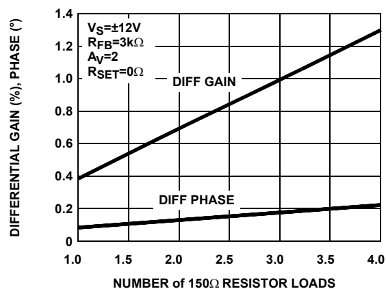
FIGURE 16. DIFFERENTIAL GAIN/PHASE, F_O=3.58\text{MHz} (2/3 POWER MODE)
