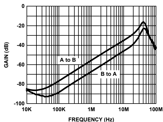
FIGURE 14. CHANNEL SEPARATION
