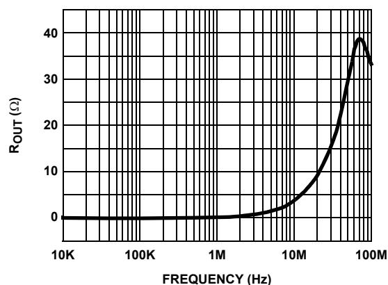
FIGURE 13. OUTPUT IMPEDANCE
