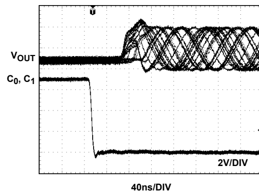
FIGURE 36. ENABLE TIME
