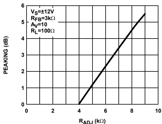
FIGURE 11. PEAKING vs R_{ADJ}
