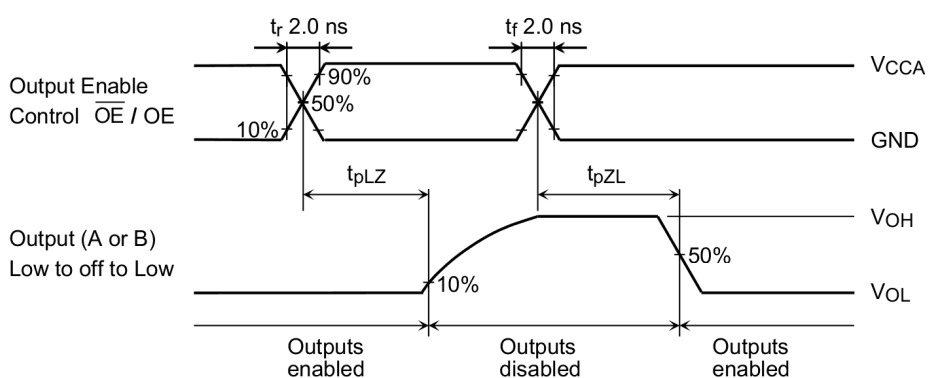
Fig. 14.4 AC Waveform of t_{PLZ} , t_{PZL}
