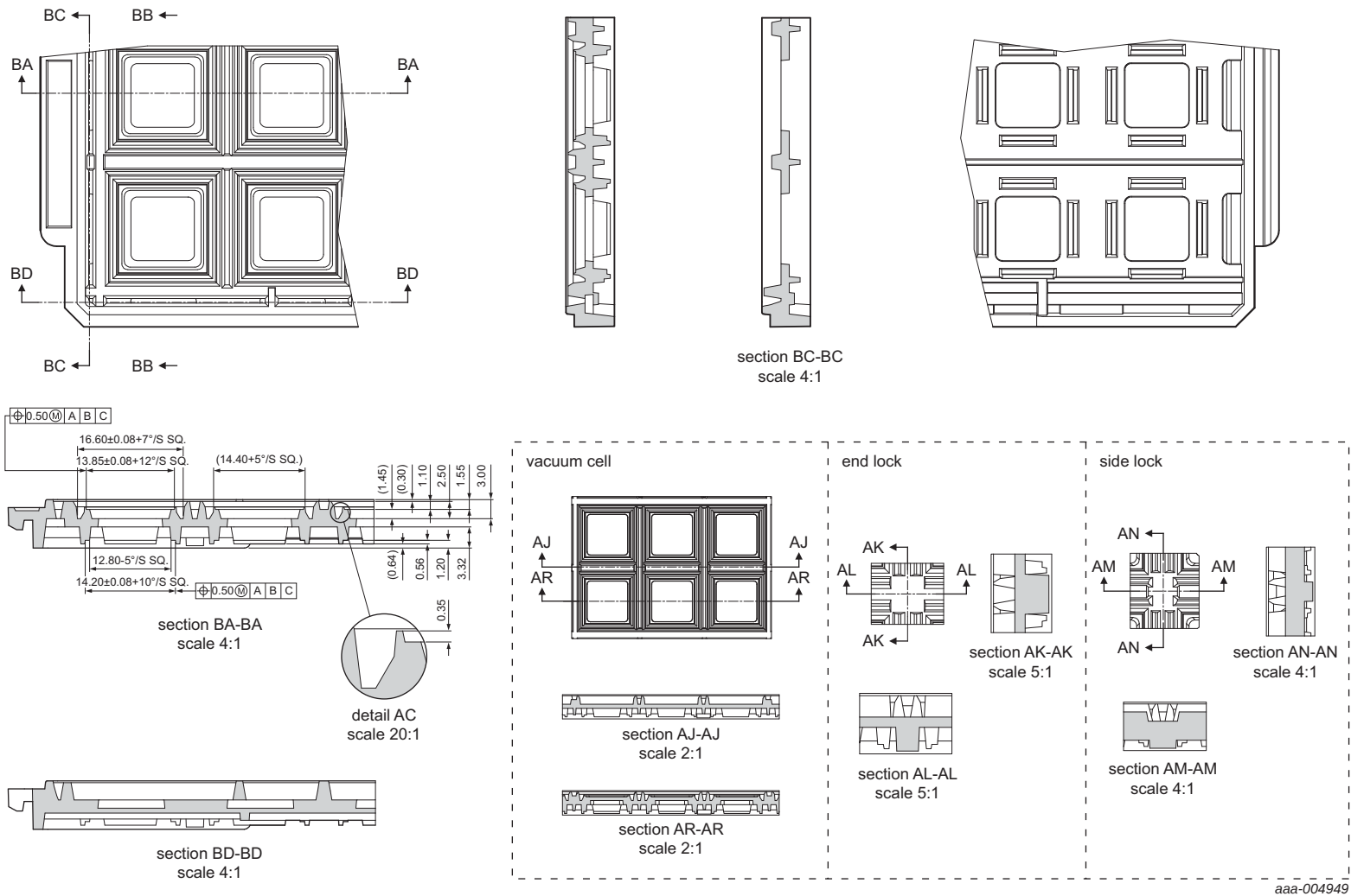
Fig 40. Tray details
