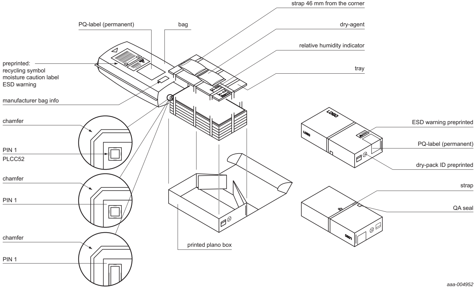
Fig 39. Packing information 5 tray
