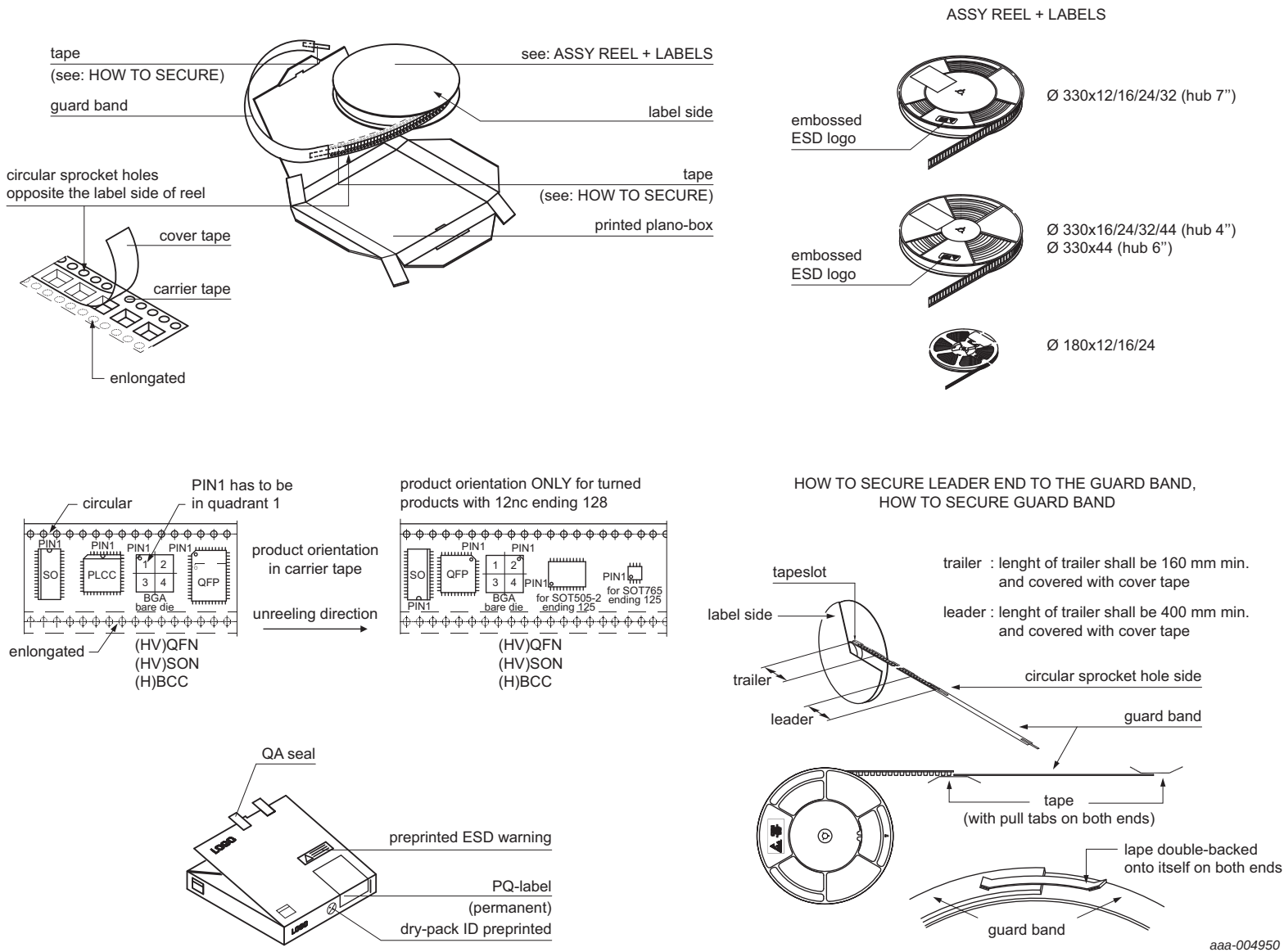
Fig 41. Packing information Reel
