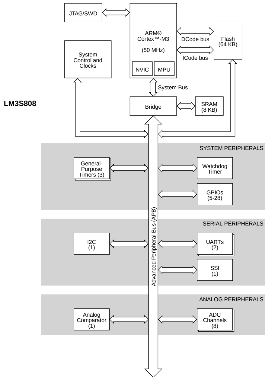
Figure 1-1. Stellaris® LM3S808 Microcontroller High-Level Block Diagram
