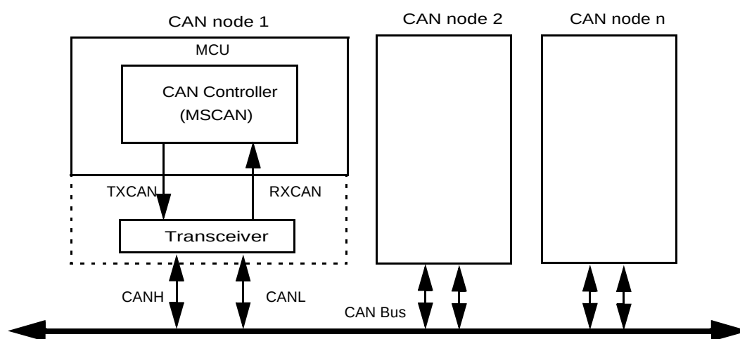
Figure 12-2. CAN System
