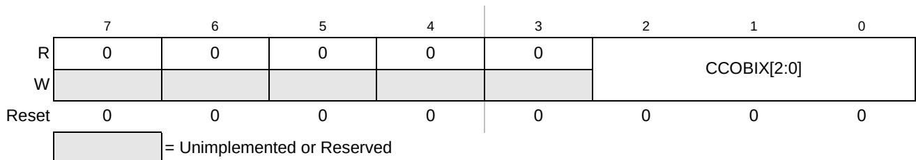
Figure 19-8. FCCOB Index Register (FCCOBIX)
