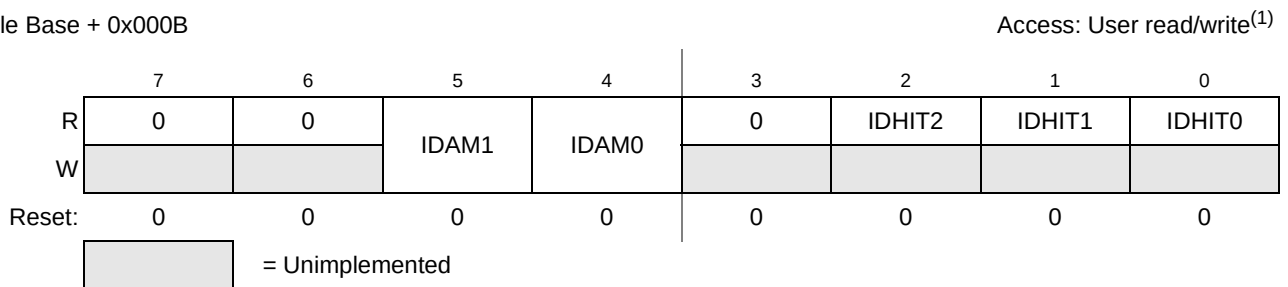
Figure 12-15. MSCAN Identifier Acceptance Control Register (CANIDAC)
