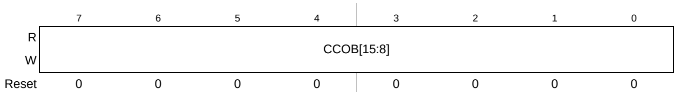
Figure 19-23. Flash Common Command Object 2 High Register (FCCOB2HI)
