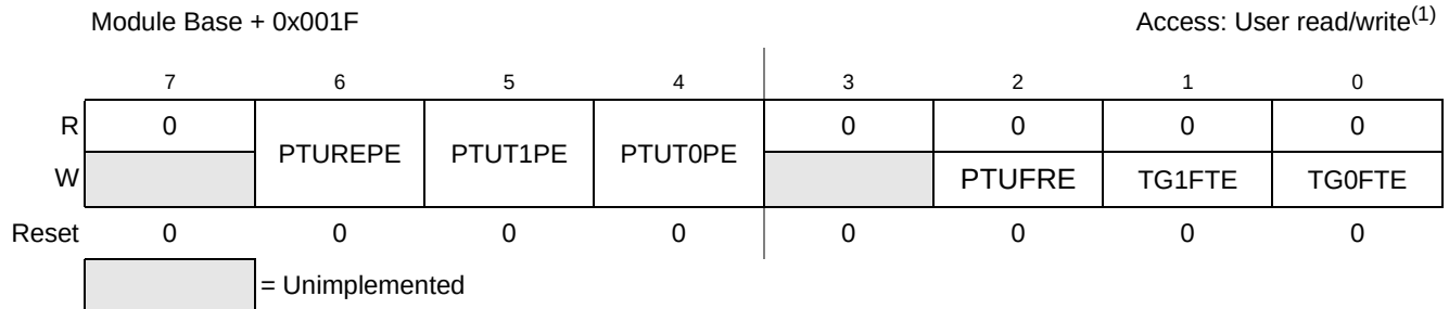
Figure 13-21. PTU Debug Register (PTUDEBUG)
