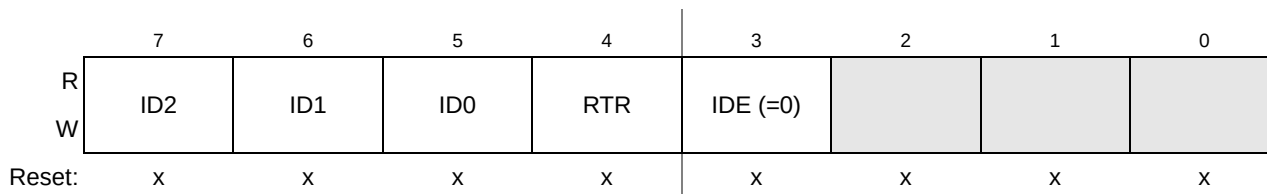
Figure 12-31. Identifier Register 1 — Standard Mapping
