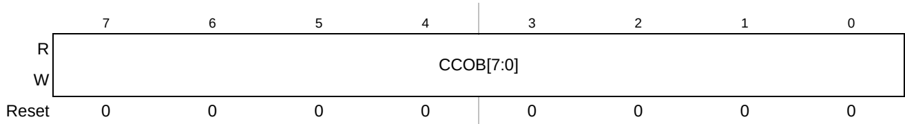
Figure 19-20. Flash Common Command Object 0 Low Register (FCCOB0LO)
