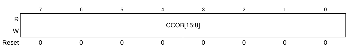
Figure 19-19. Flash Common Command Object 0 High Register (FCCOB0HI)
