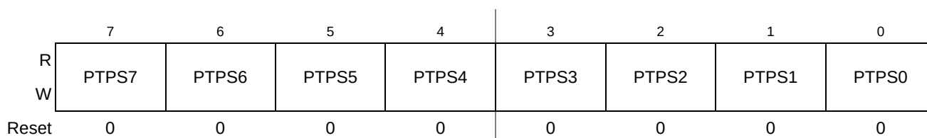
Figure 11-21. Precision Timer Prescaler Select Register (PTPSR)
