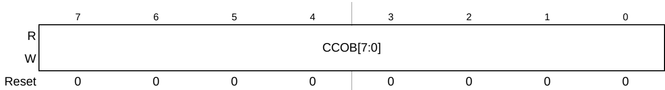
Figure 19-30. Flash Common Command Object 5 Low Register (FCCOB5LO)
