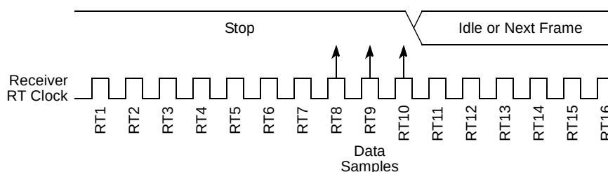
Figure 15-29. Fast Data
