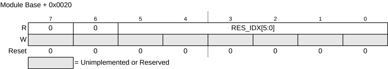
Figure 9-24. ADC Result Index Register (ADCRIDX)
