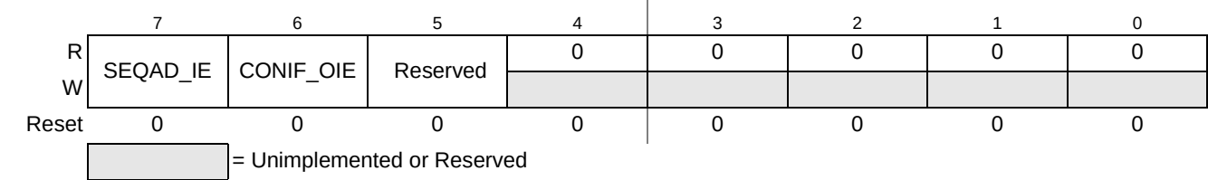
Figure 9-11. ADC Interrupt Enable Register (ADCIE)
