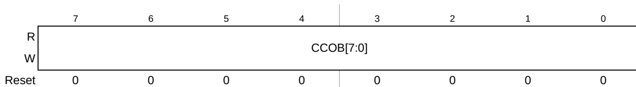
Figure 19-26. Flash Common Command Object 3 Low Register (FCCOB3LO)
