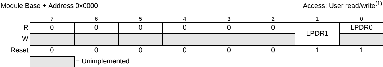
Figure 18-3. Port LP Data Register (LPDR)
