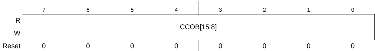
Figure 19-21. Flash Common Command Object 1 High Register (FCCOB1HI)
