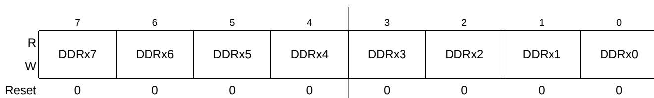
Figure 2-13. Data Direction Register
