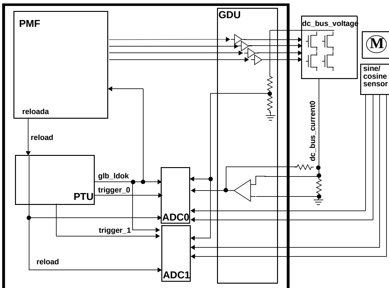
Figure 1-10. BDCM Control Loop Configuration
