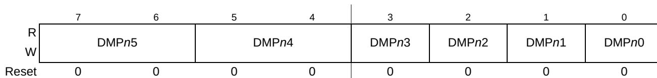
Figure 14-39. PMF Disable Mapping Register (PMFDMP0-5)
