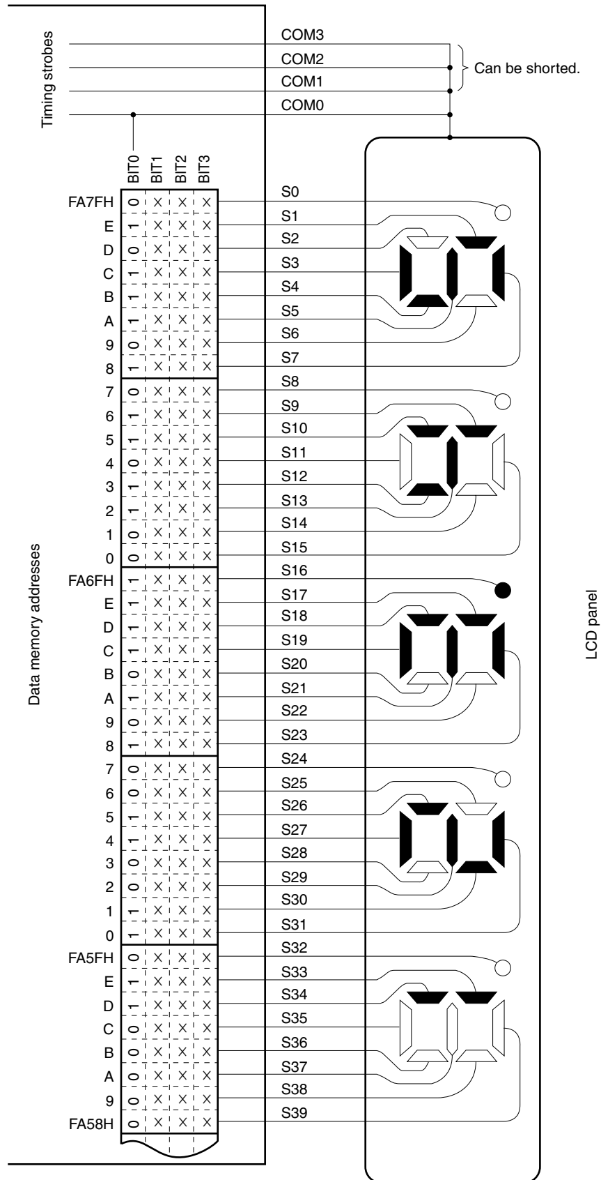
Figure 19-12. Static LCD Panel Connection Example
