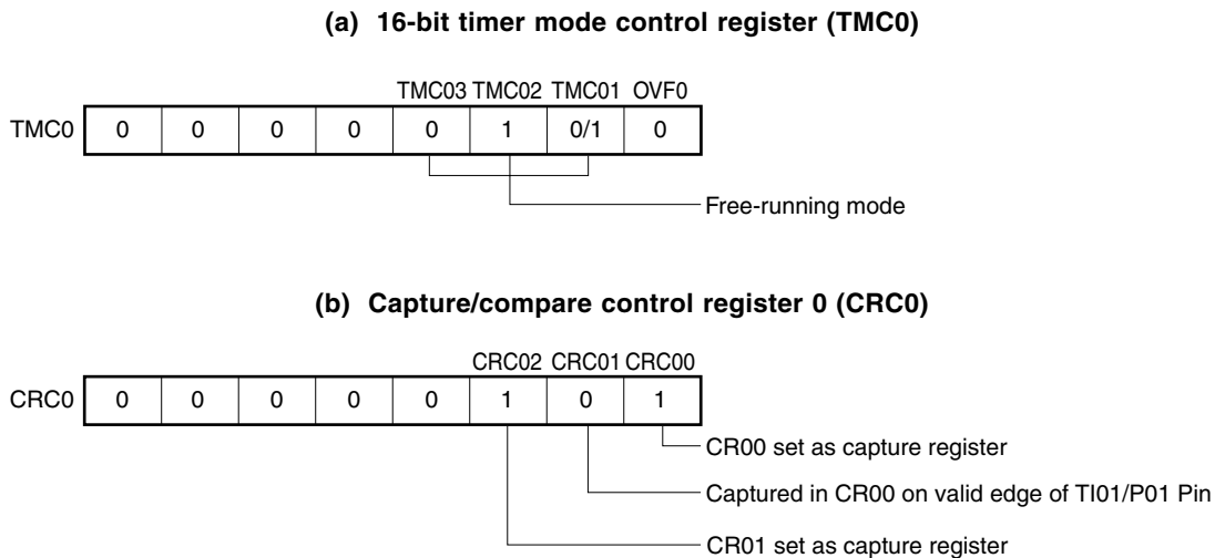
Figure 8-20. Control Register Settings for Two Pulse Width Measurements with Free-Running Counter
