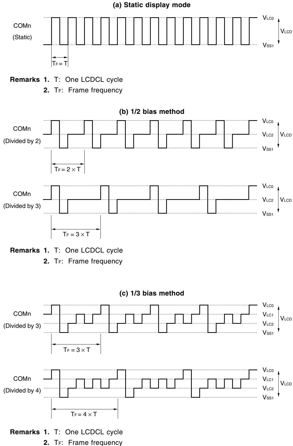
Figure 19-6. Common Signal Waveform
