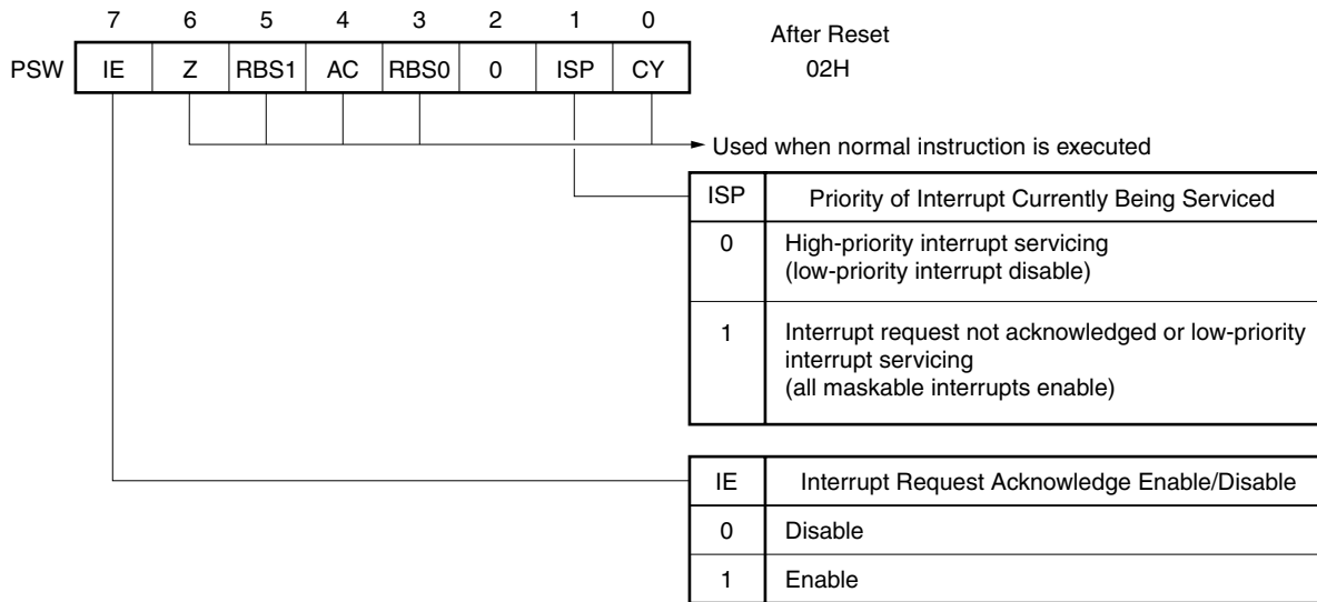
Figure 20-9. Program Status Word Format
