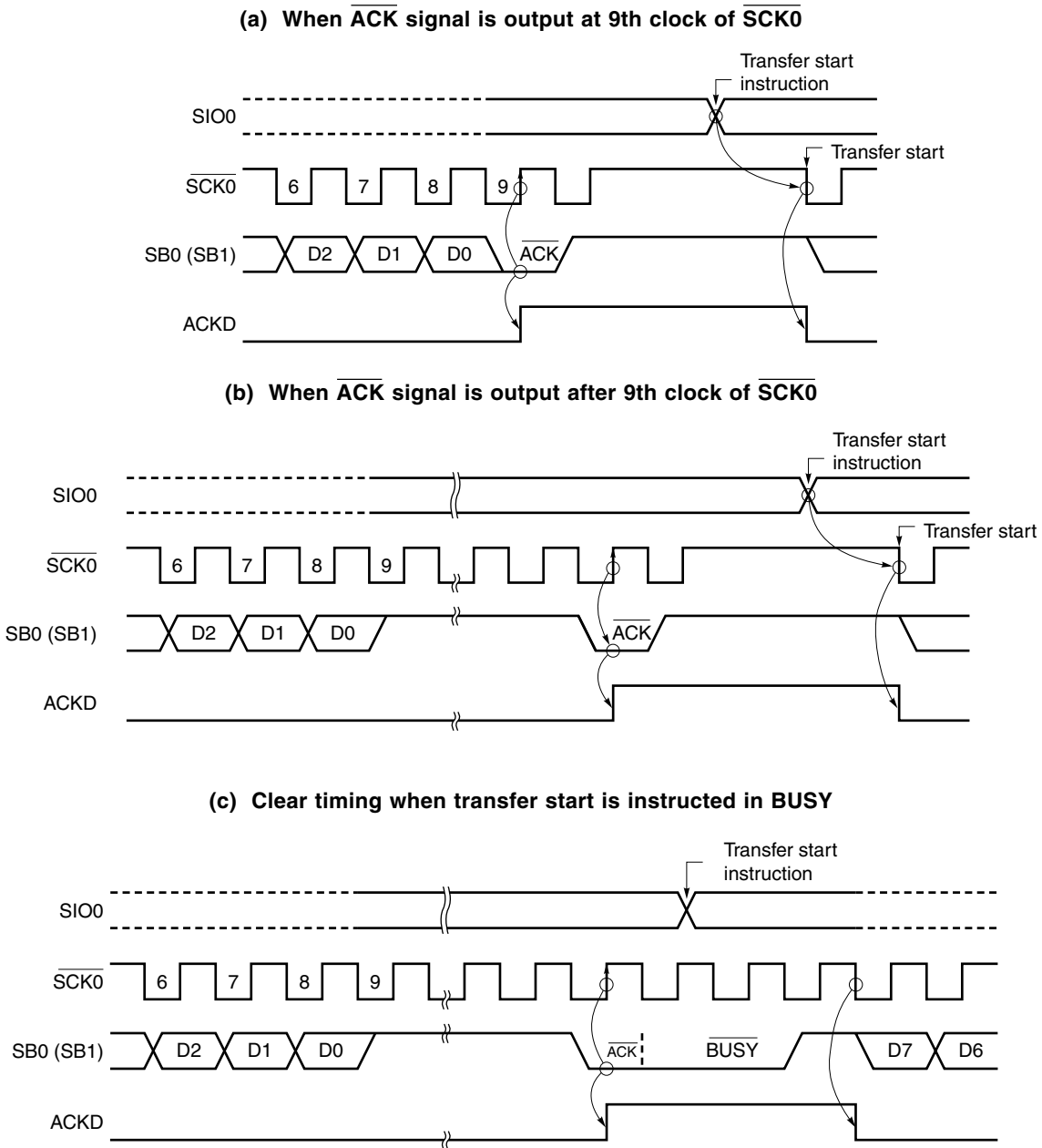
Figure 15-25. BSYE Operation
