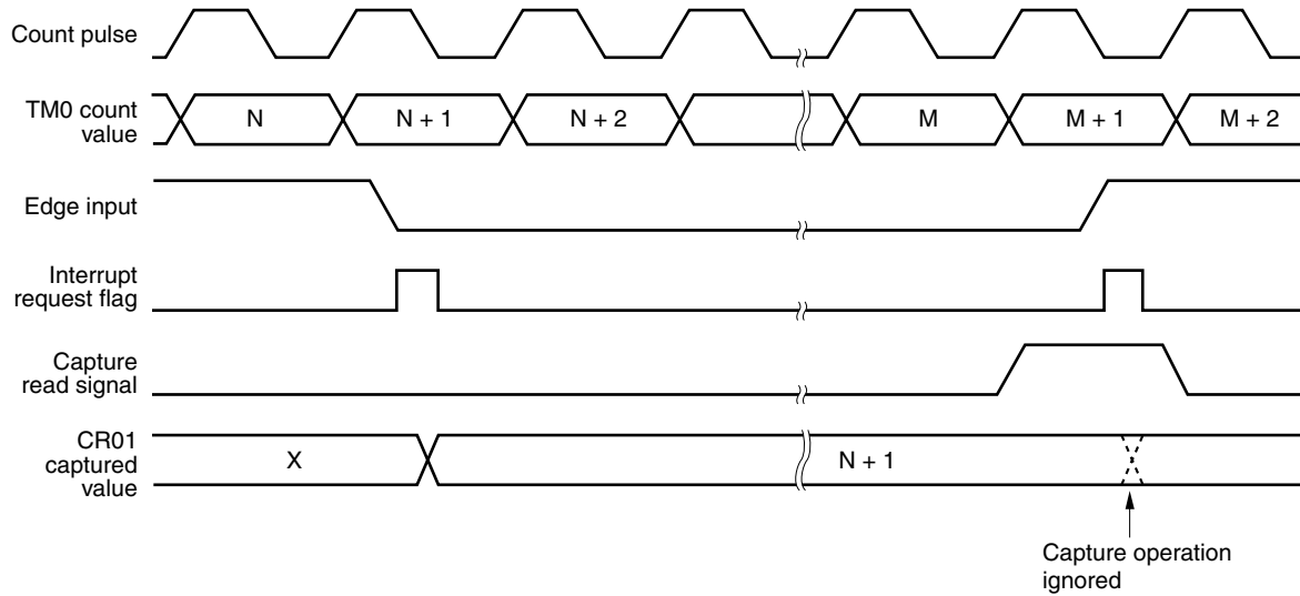
Figure 8-37. Capture Register Data Retention Timing
