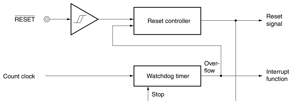
Figure 22-1. Block Diagram of Reset Function
