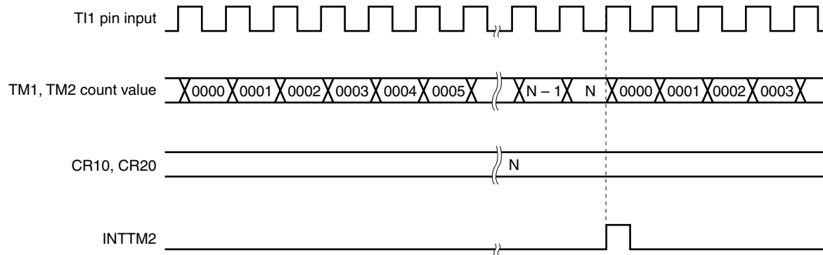
Figure 9-12. External Event Counter Operation Timings (with Rising Edge Specified)
