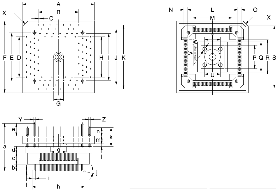
Figure A-2. TGC-100SDW Note Drawing (For Reference Only)
