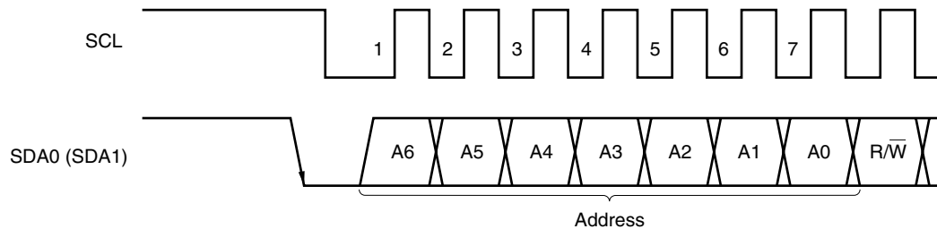
Figure 16-16. Address
