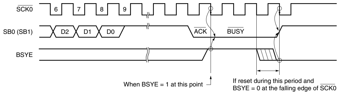
Figure 15-25. BSYE Operation
