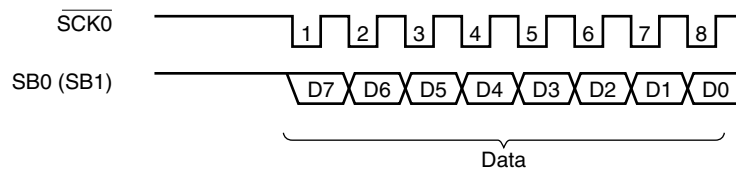
Figure 15-17. Data
