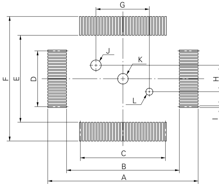
Figure A-4. EV-9200GF-100 Footprint (For Reference Only)
