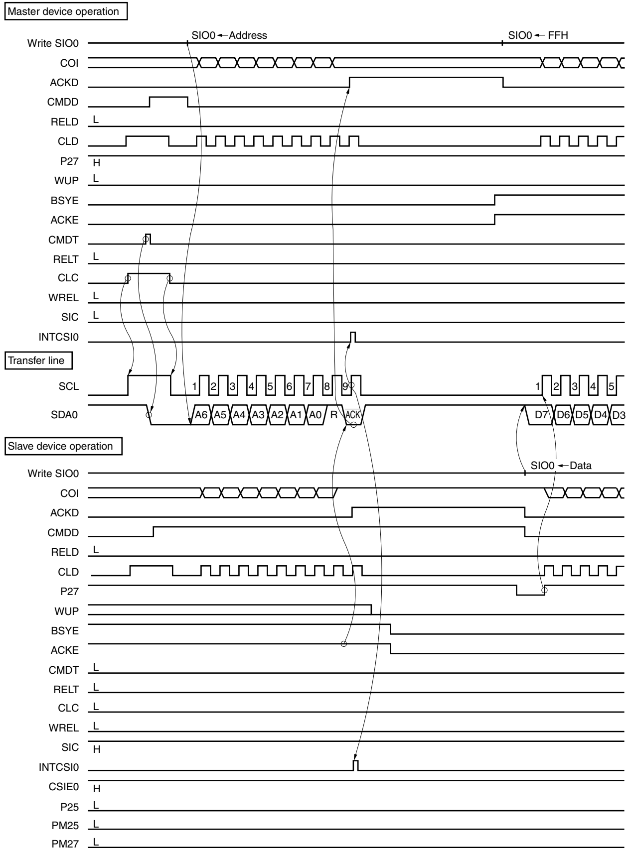
Figure 16-23. Data Transmission from Slave to Master (Both Master and Slave Selected 9-Clock Wait) (1/3) (a) Start condition to address
