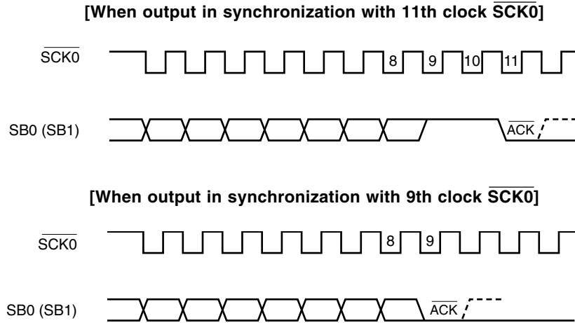
Figure 15-18. Acknowledge Signal
