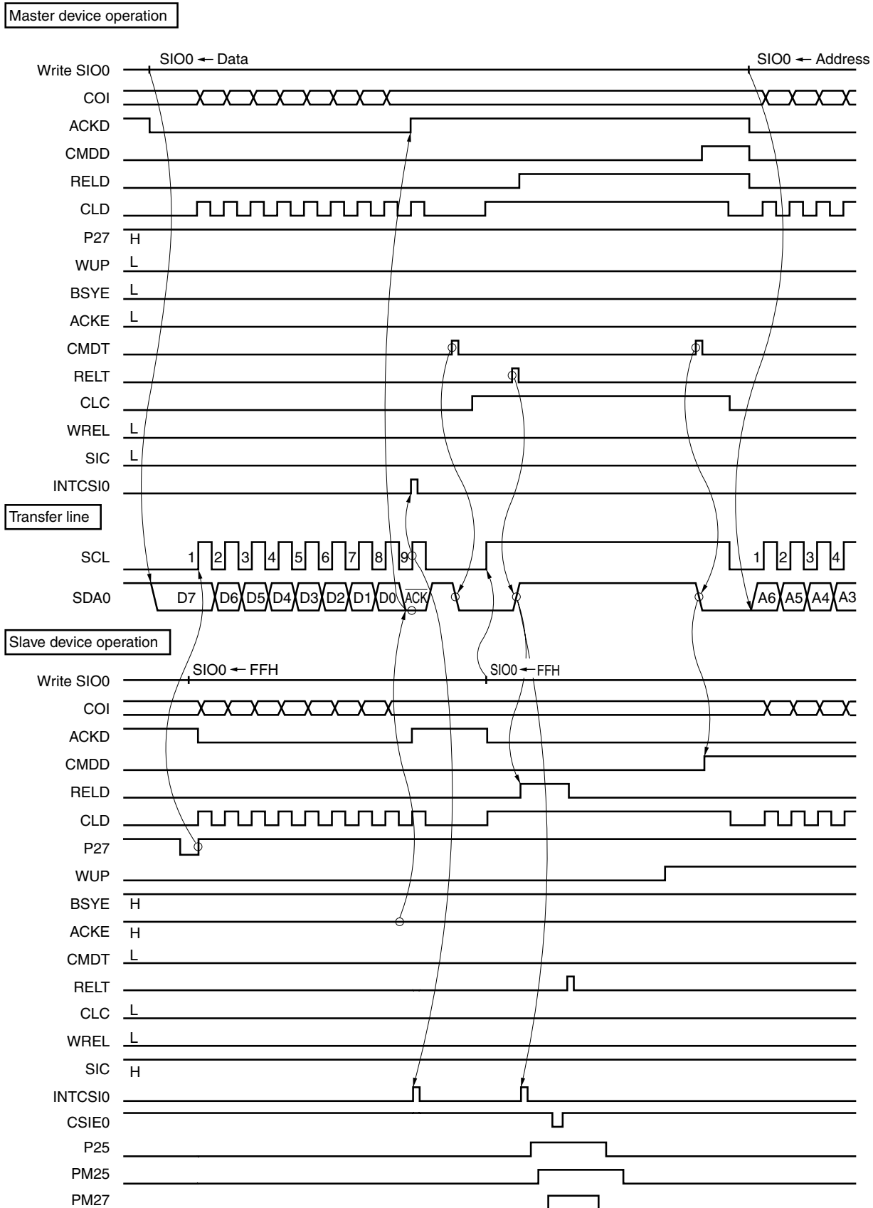
Figure 16-22. Data Transmission from Master to Slave (Both Master and Slave Selected 9-Clock Wait) (3/3) (c) Stop condition
