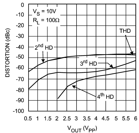
Harmonic Distortion vs. V_{\text{OUT}} @ 5MHz
