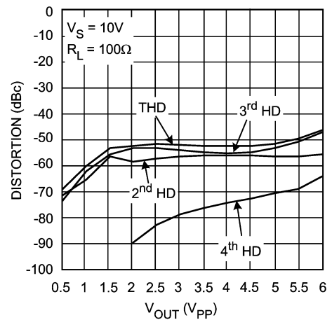
Harmonic Distortion vs. V_{\text{OUT}} @ 20MHz
