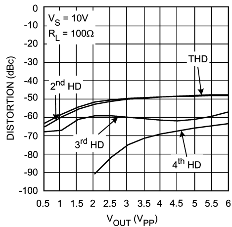
Harmonic Distortion vs. V_{\text{OUT}} @ 10MHz
