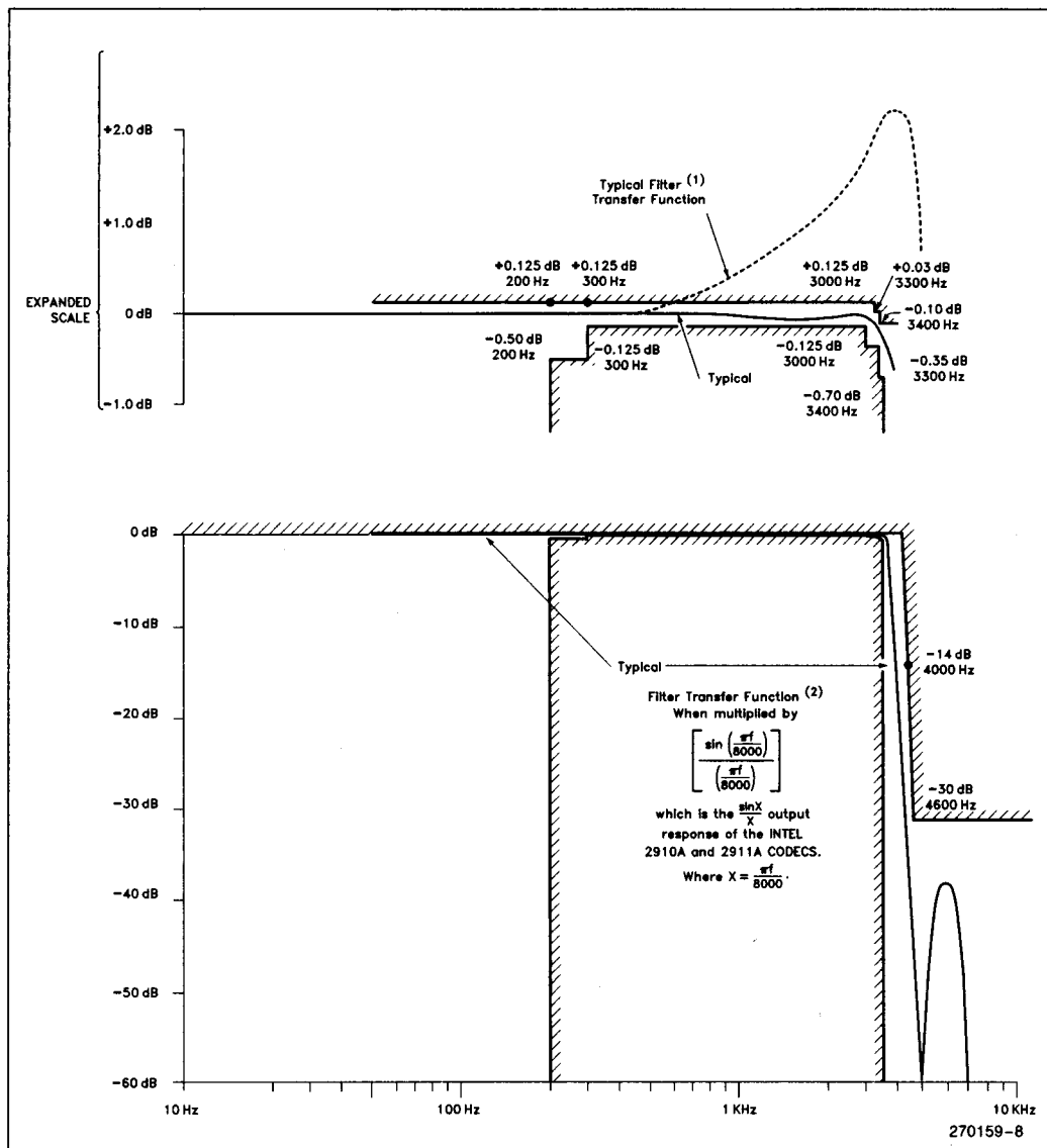
Figure 8. Receive Filter
