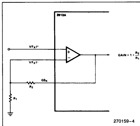
Figure 4. Transmit Filter Gain Adjustment
