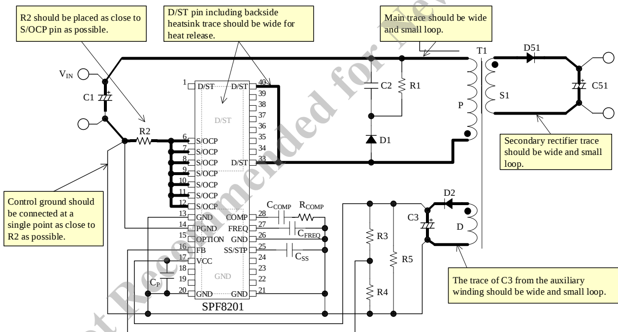
Figure 10-4. Peripheral Circuit Example around the IC
