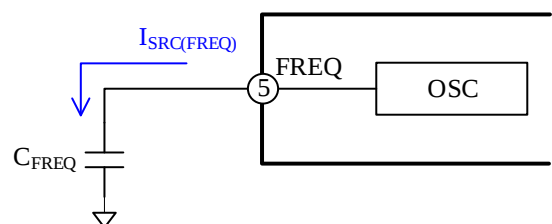
Figure 9-9. FREQ Pin Peripheral Circuit
