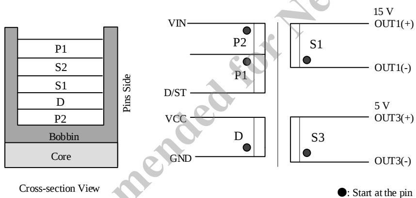
Figure 12-1. Winding Structure
