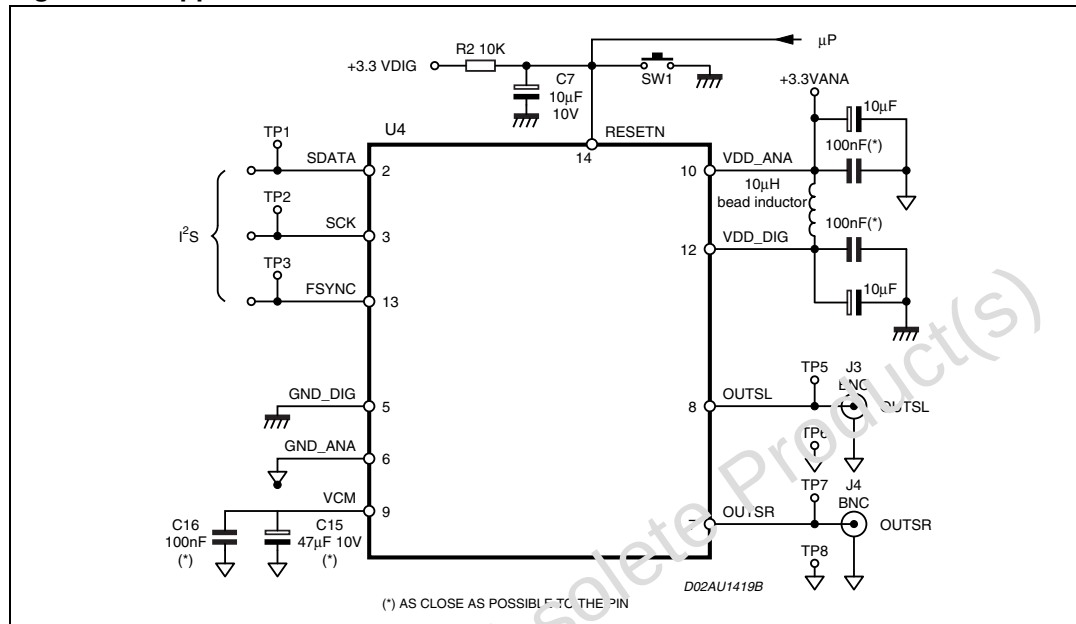
Figure 7. Application circuit
