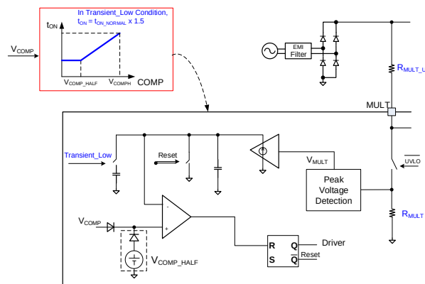
Figure 6: On-Time Generation
