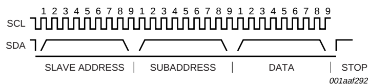
Fig 13. I 2 C-bus access
