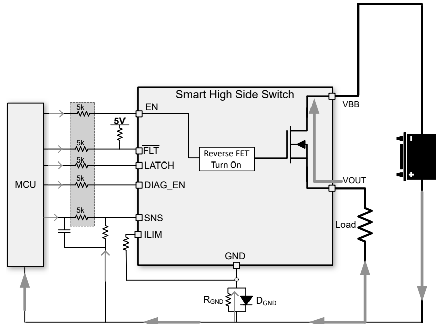
Figure 8-24. MCU I/O Protections
