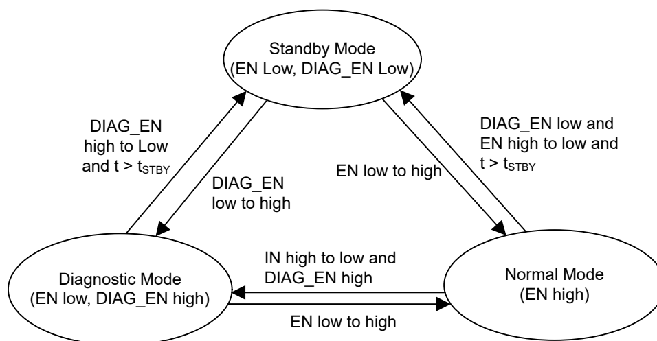
Figure 8-25. Work Mode State Machine
