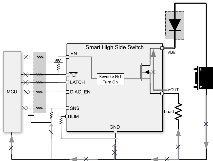
Figure 8-22. Reverse Protection with Blocking Diode
