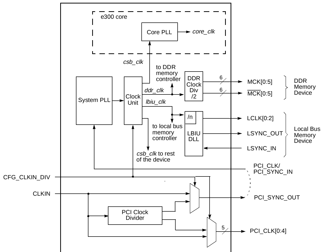
Figure 61. MPC8379E Clock Subsystem
