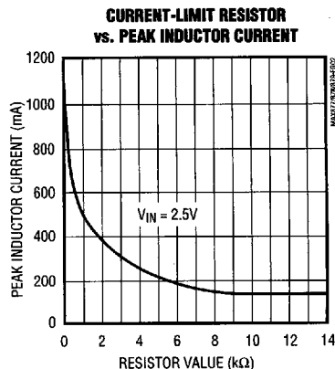
Figure 2. Current-Limit Resistor vs. Peak Inductor Current
