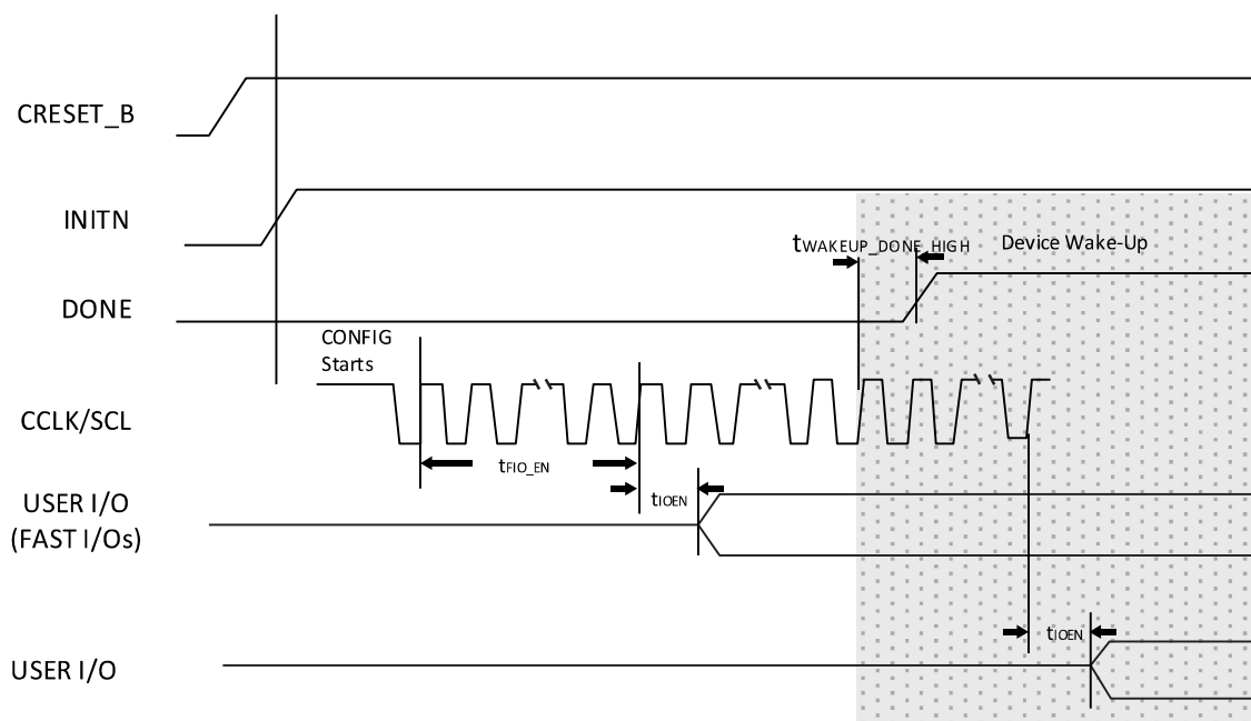
Figure 4.22. Slave SPI/I²C/I3C Wake-Up Timing
