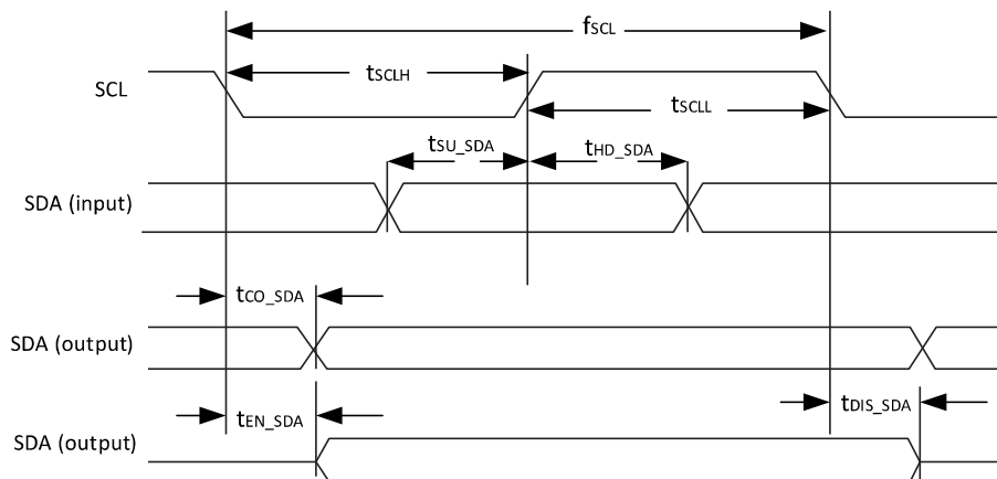
Figure 4.20. I²C /I³C Configuration Timing
