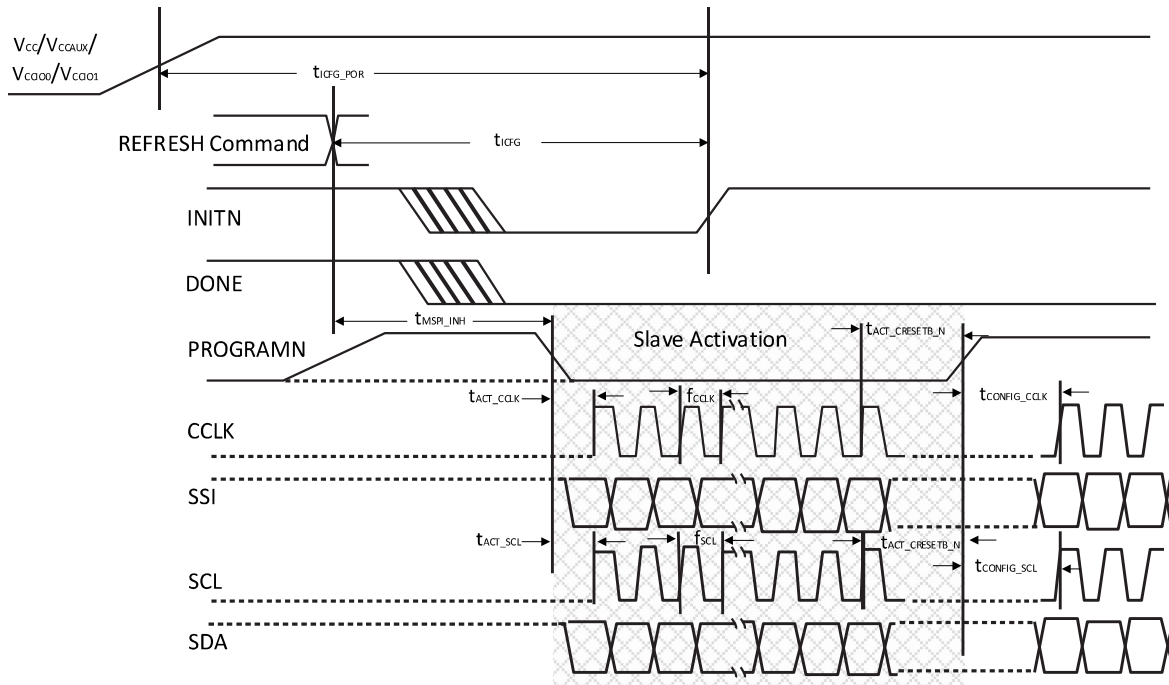
Figure 4.15. Slave SPI/I²C/I³C POR/REFRESH Timing
