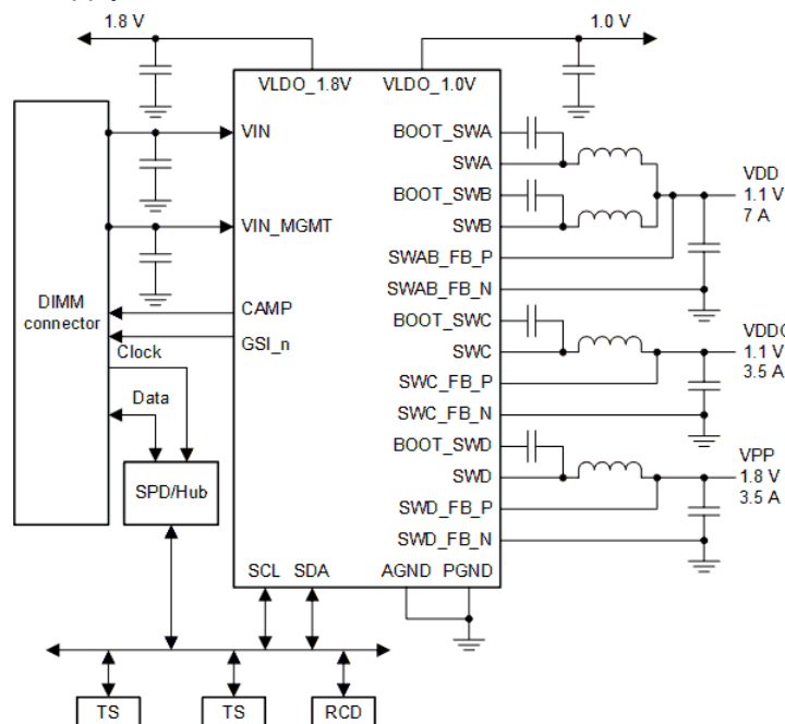
Figure 3-1. Simplified Application
