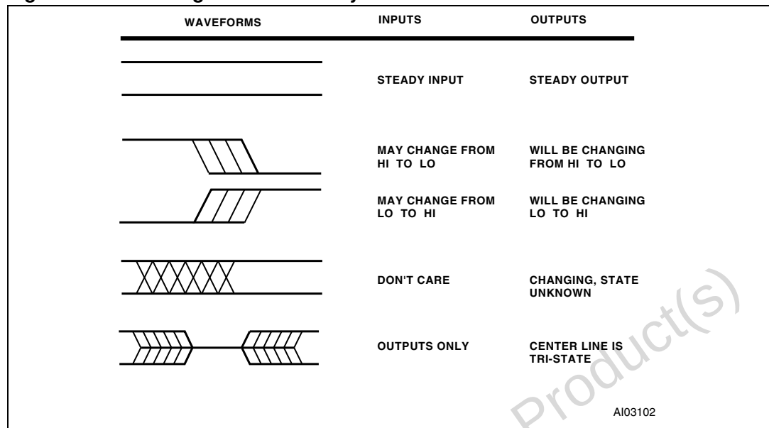
Figure 36. Switching waveforms – key
