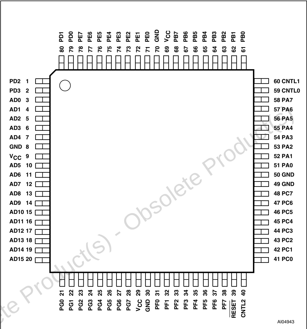
Figure 1. LQFP80 connections
