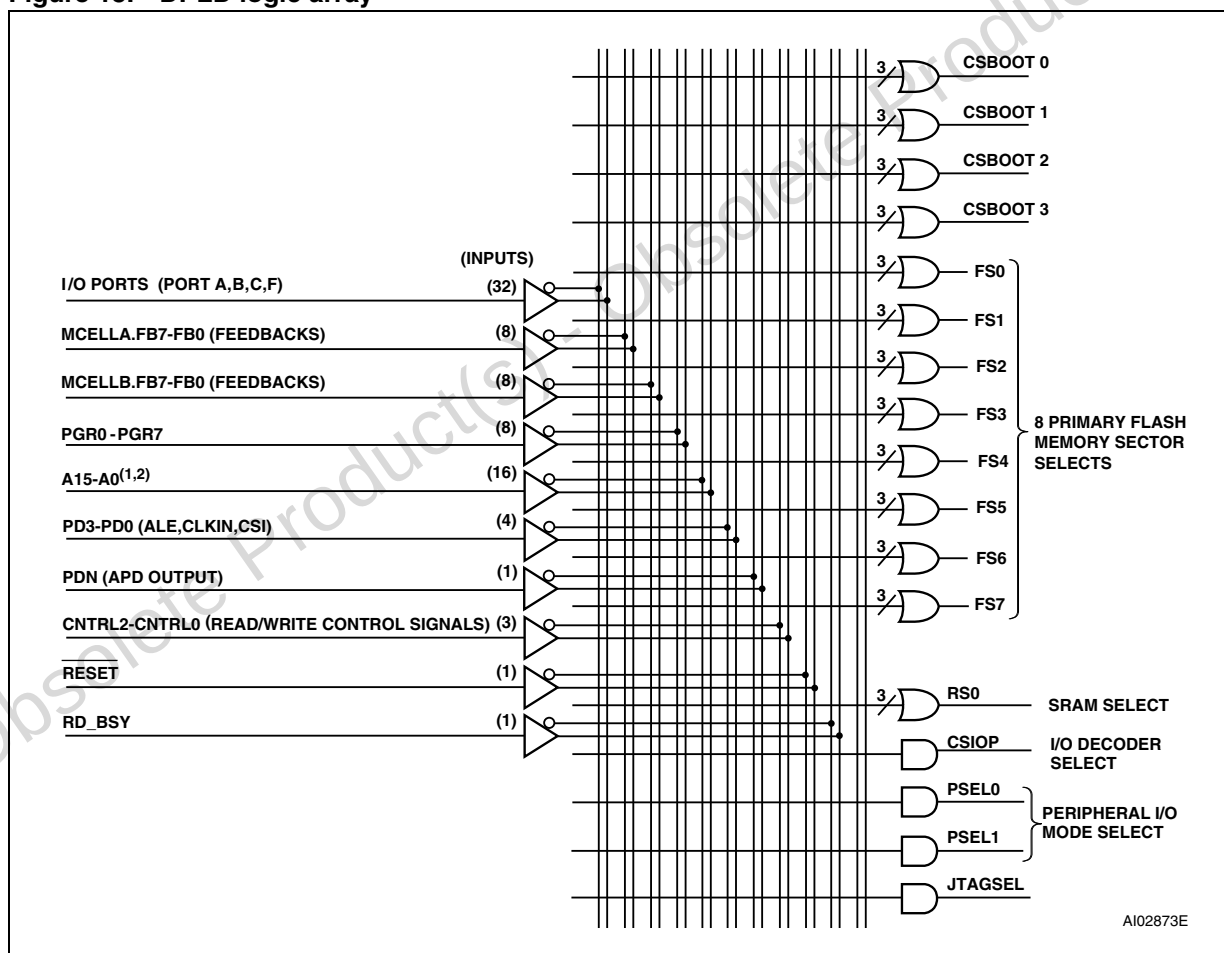
Figure 13. DPLD logic array
