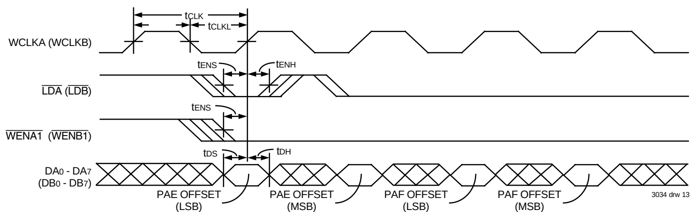
Figure 12. Write Offset Register Timing
