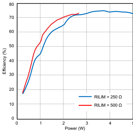
Figure 8-1. Rectifier Efficiency
