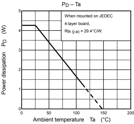
TC78B042FTG (QFN32)
