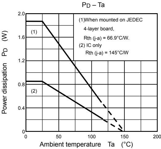
TC78B041FNG (SSOP30)
