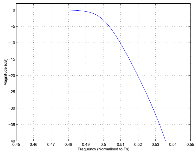
Figure 9-5. Transition Band (Detail)—DAC, F_{s_{int}} = 44.118 kHz
