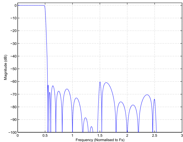
Figure 9-3. Stopband—DAC, F_{s_{int}} = 44.118 kHz
