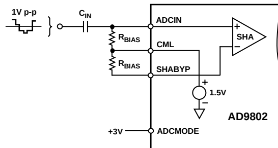
Figure 23. AC-Coupled Input
