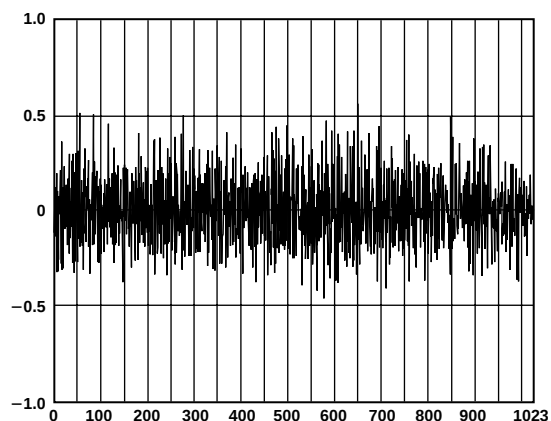
Figure 28. Direct ADC-Mode Typical DNL
