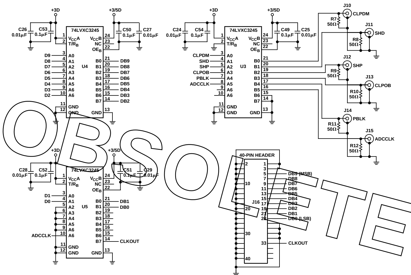
Figure 33. Evaluation Board
