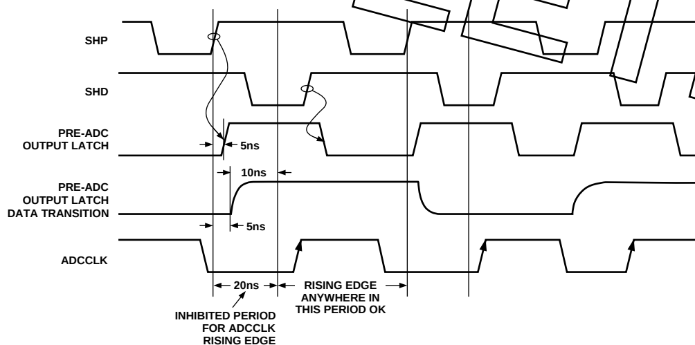
Figure 13. ADCCLK Timing Edge
