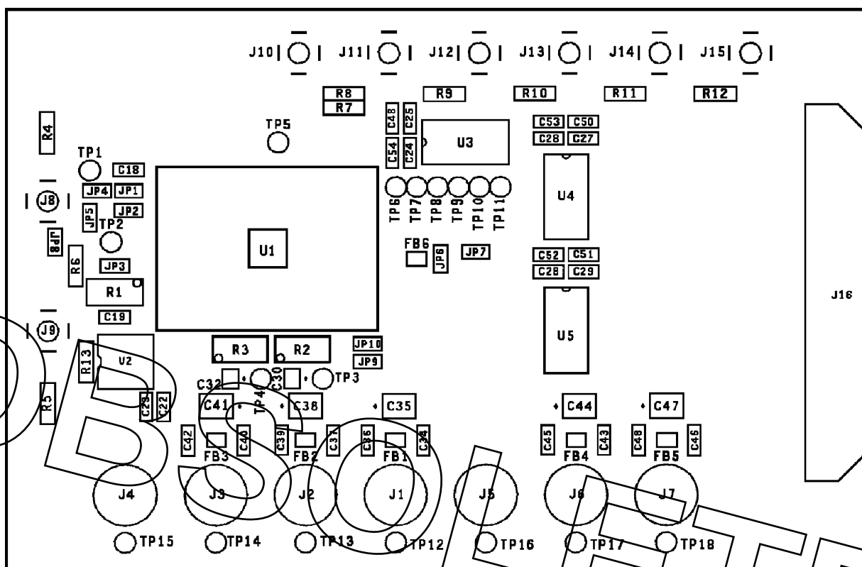
Figure 38. Primary Side Assembly
