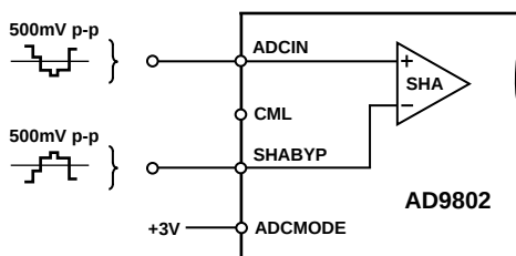
Figure 25. Differential Input
