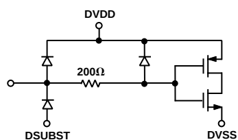
Figure 3. Pin 16 (ADCCLK)
