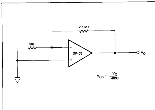
TYPICAL OFFSET VOLTAGE TEST CIRCUIT
