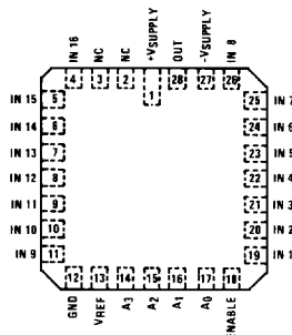
HI4-546/883 (CERAMIC LCC) TOP VIEW
