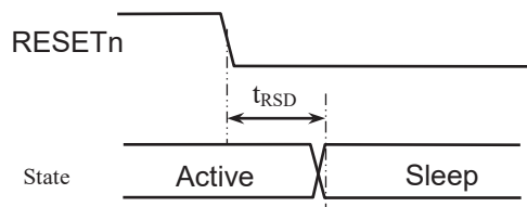
Figure 3a: Transition to Sleep (RESETn)
