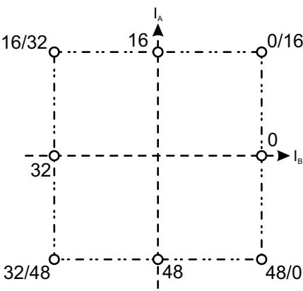
Figure 12: Uncompensated Half-Step Phase Diagram
