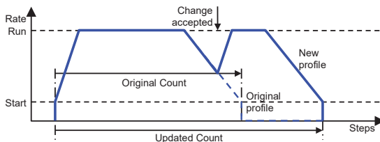
Figure 22b: Count Decrease (late)
