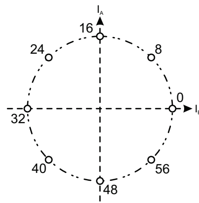
Figure 11: Compensated Half-Step Phase Diagram
