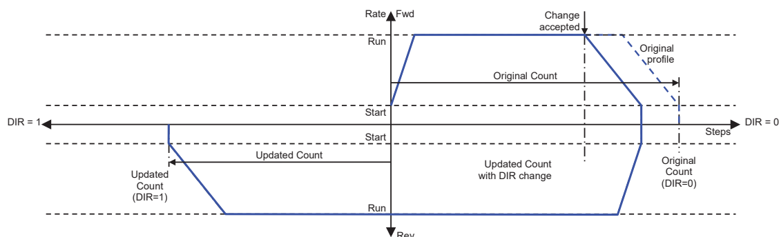
Figure 23: Direction Change
