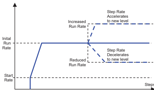
Figure 20: Run Speed Change
