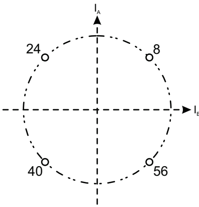
Figure 10: Full-Step 2-Phase Drive Phase Diagram
