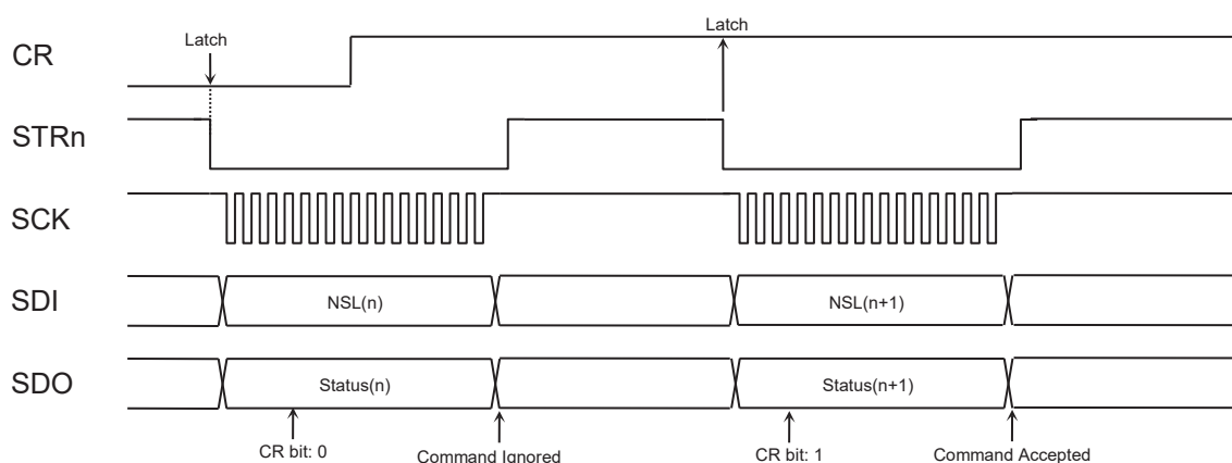
Figure 24: Motion Profile Update with CR Status Checking
