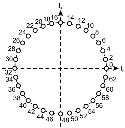
Figure 14: Eighth-Step Phase Diagram
