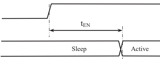
Figure 3b: Transition from Sleep (RESETn)
