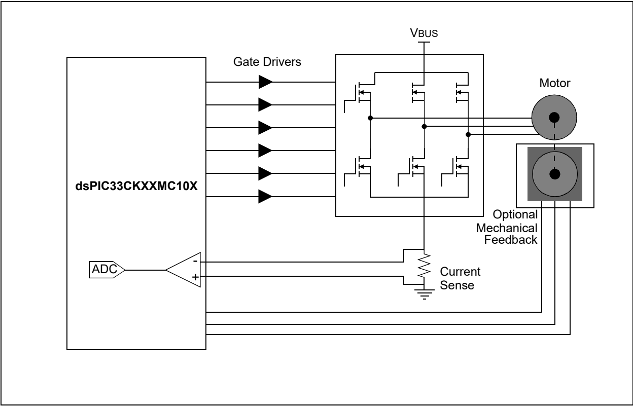
FIGURE 2-6: BLDC MOTOR
