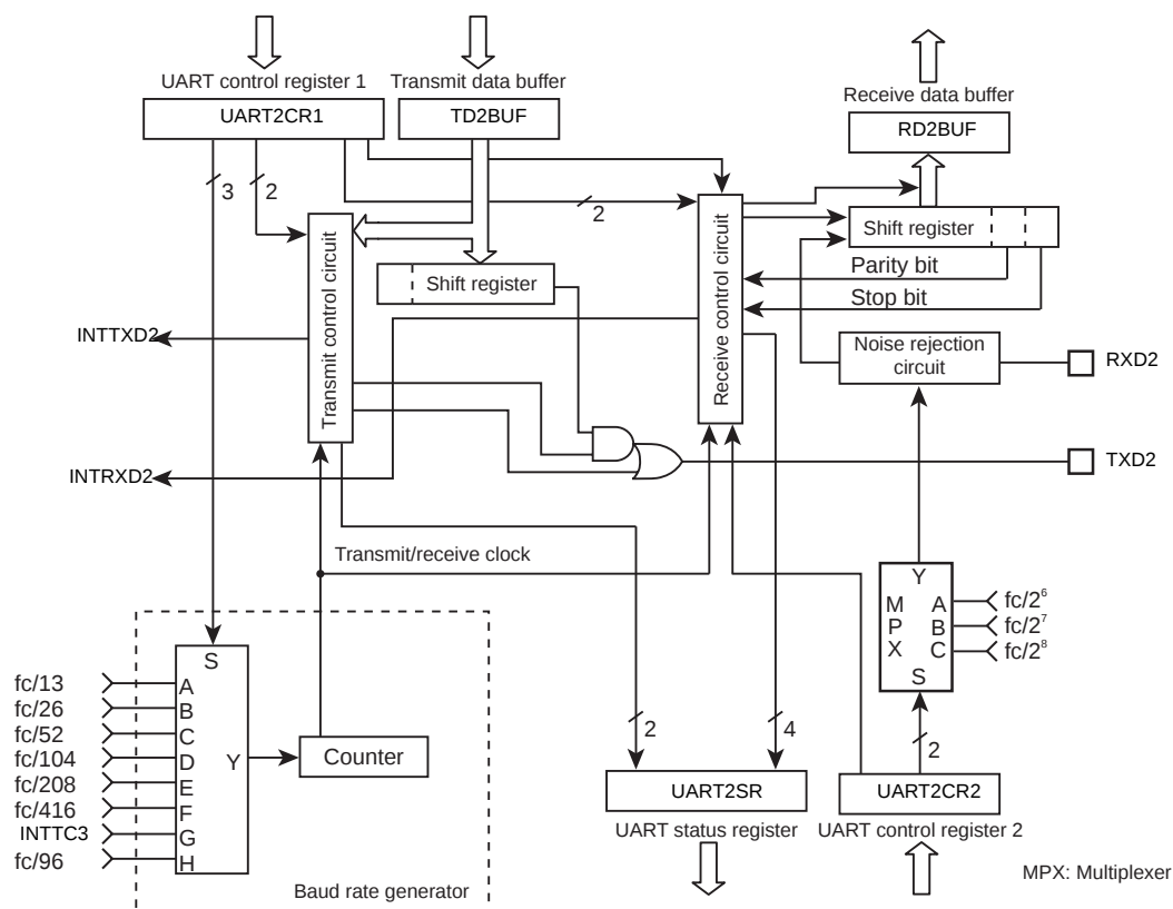
Figure 13-1 UART2 (Asynchronous Serial Interface)
