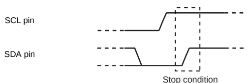
Figure 15-6 Stop Condition Generation
