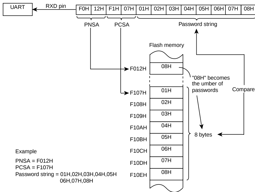
Figure 19-5 Password Comparison
