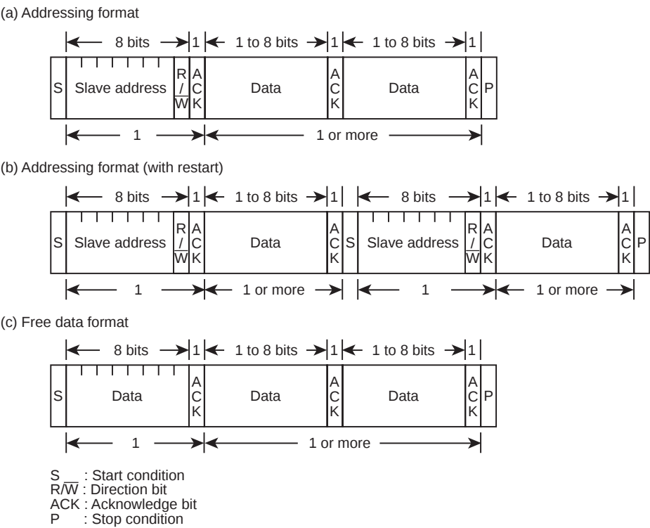
Figure 15-2 Data Format in of I 2 C Bus
