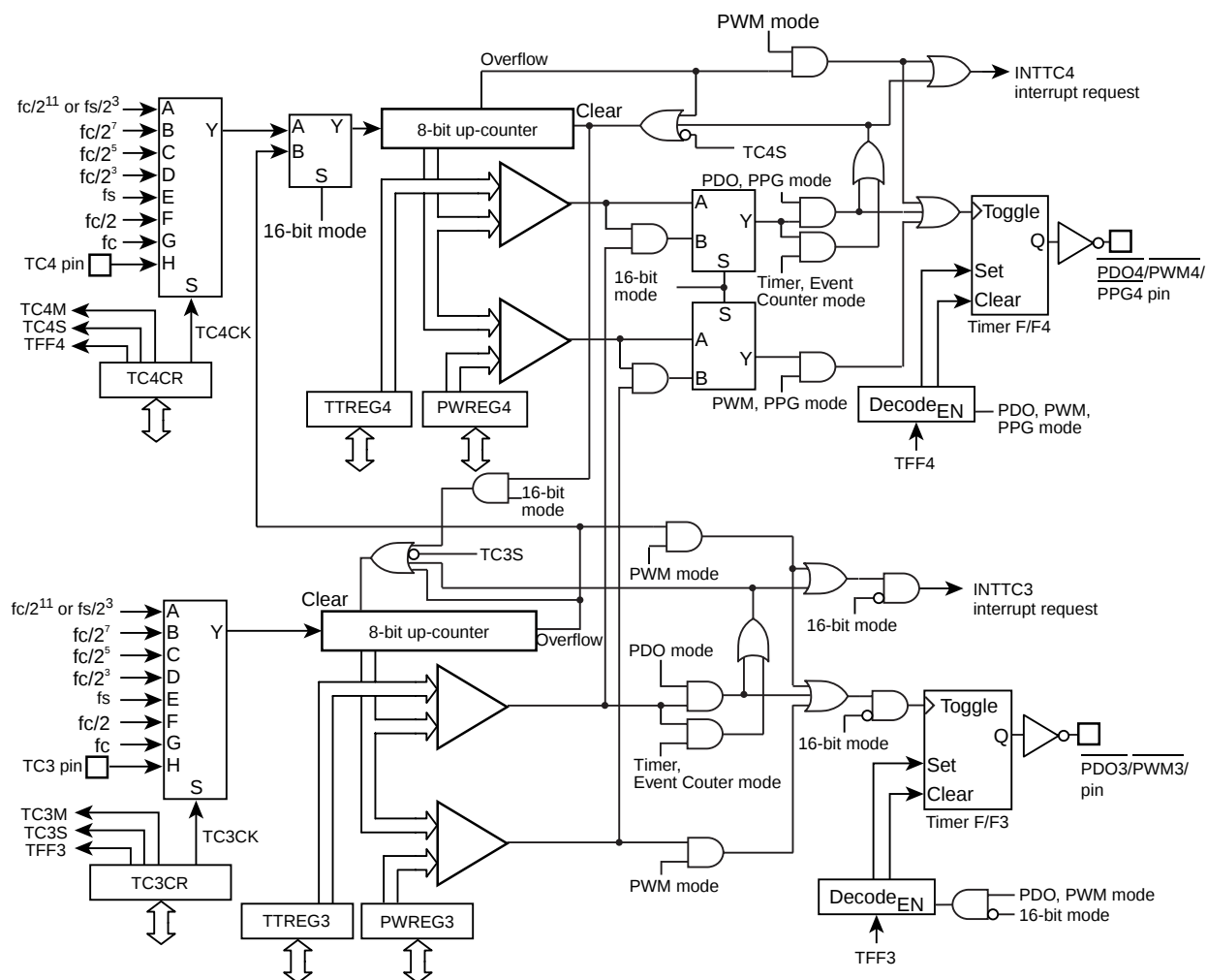
Figure 11-1 8-Bit TimerCounter 3, 4
