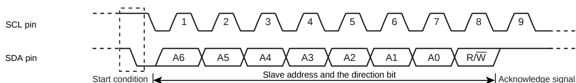
Figure 15-5 Start Condition Generation and Slave Address Generation
