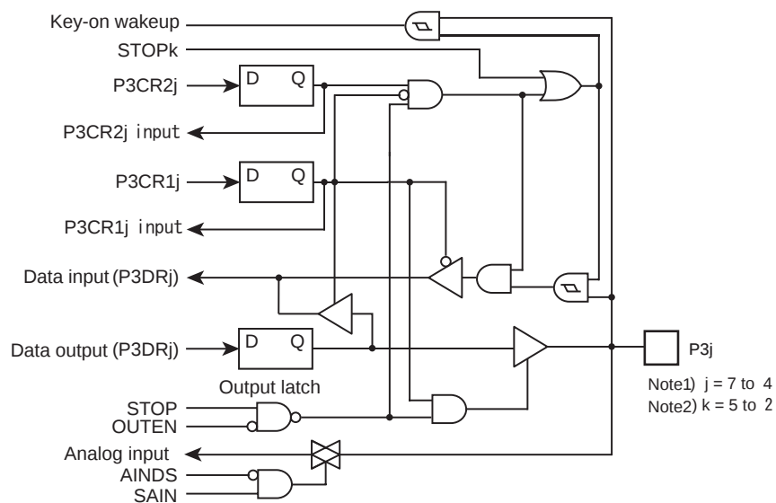
c) Equivalent circuit of P34 to P37
