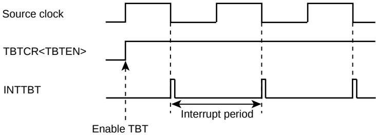
Figure 9-2 Time Base Timer Interrupt
