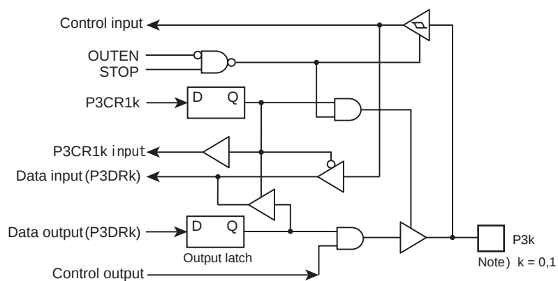
a) Equivalent circuit of P30, P31
