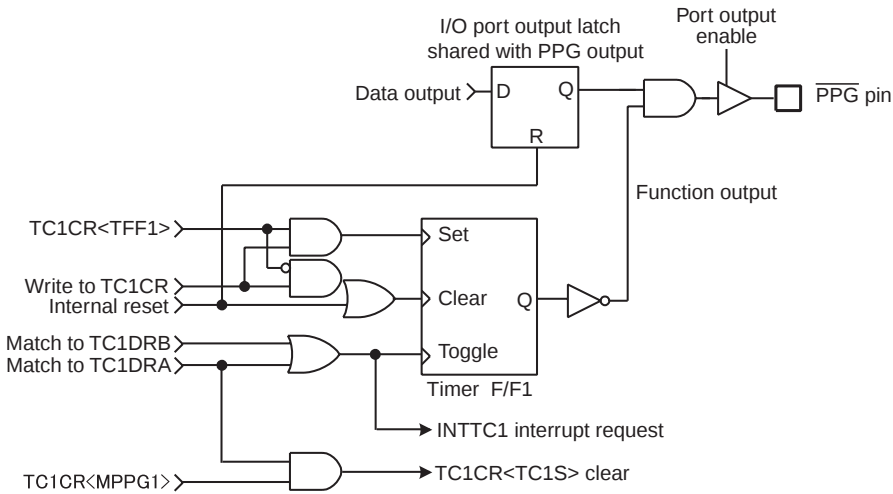
Figure 10-7 PPG Output
