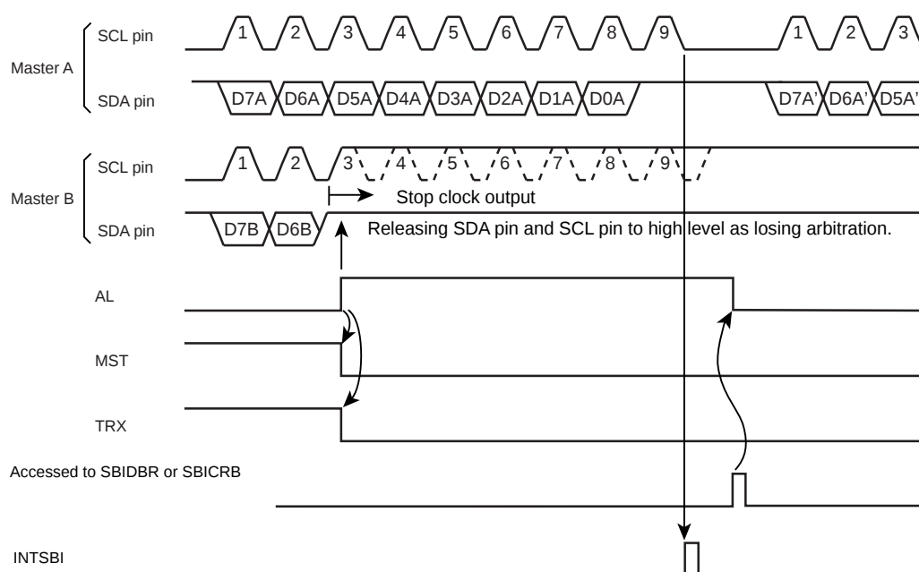
Figure 15-8 Example of when a Serial Bus Interface Circuit is a Master B
