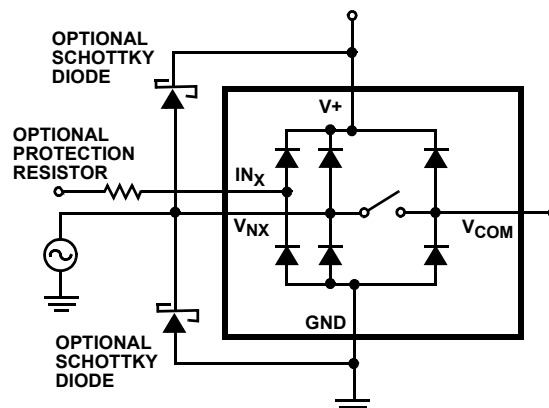
FIGURE 6. OVERVOLTAGE PROTECTION
