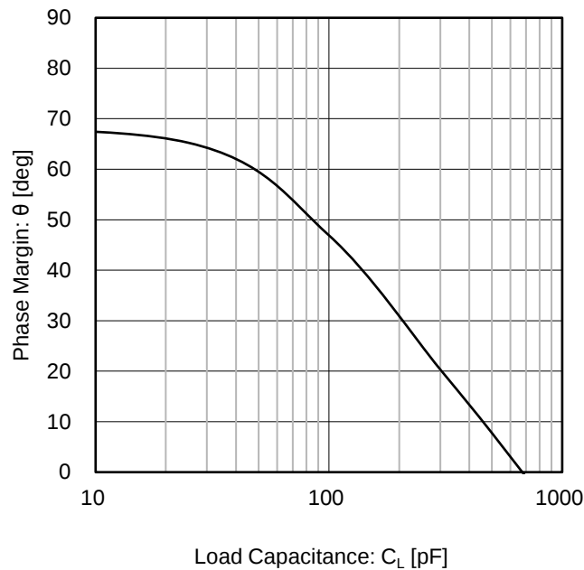
Figure 22. Phase Margin vs Load Capacitance ( V_S = 5\text{ V} , R_F = 10\text{ k}\Omega , G = 40\text{ dB} )
