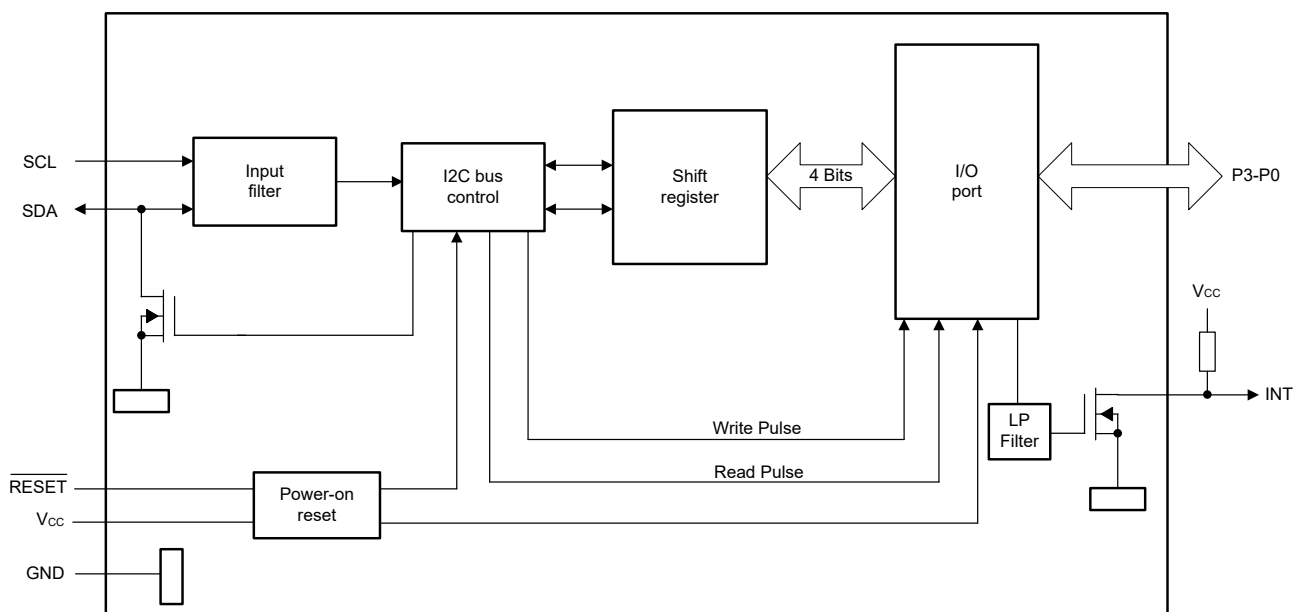
Figure 8-1. Logic Diagram
